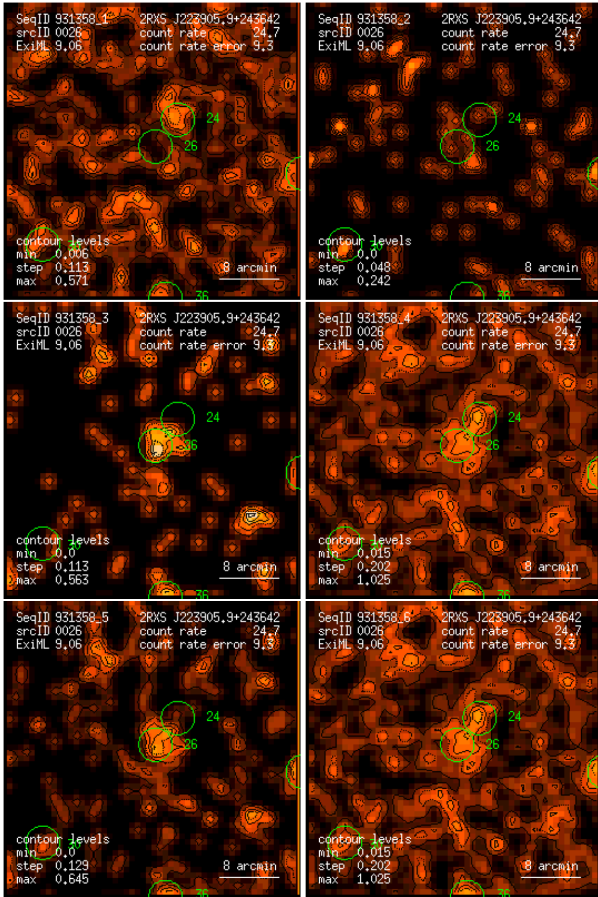
Figure 26: RASS 931358: detection 0026: band rate images, Gaussian filter: (1) PSPC channels 11 – 41, (2) 52 – 90, (3) 91 – 201, (4) 11 – 235, (5) 52 – 201, (6) 11 – 201. Broad band rates in counts/ks. Band rate contour levels in counts/ks/arcmin 2 .
