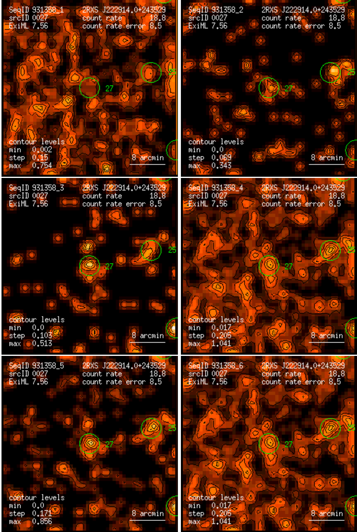
Figure 27: RASS 931358: detection 0027: band rate images, Gaussian filter: (1) PSPC channels 11 – 41, (2) 52 – 90, (3) 91 – 201, (4) 11 – 235, (5) 52 – 201, (6) 11 – 201. Broad band rates in counts/ks. Band rate contour levels in counts/ks/arcmin 2 .
