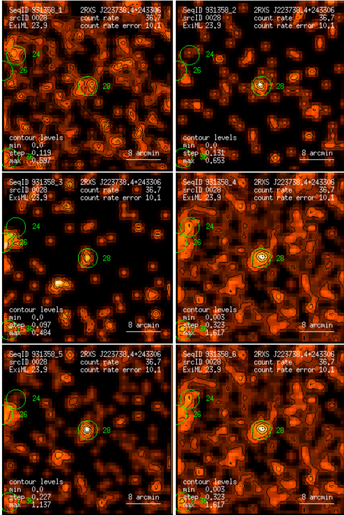
Figure 28: RASS 931358: detection 0028: band rate images, Gaussian filter: (1) PSPC channels 11 – 41, (2) 52 – 90, (3) 91 – 201, (4) 11 – 235, (5) 52 – 201, (6) 11 – 201. Broad band rates in counts/ks. Band rate contour levels in counts/ks/arcmin 2 .
