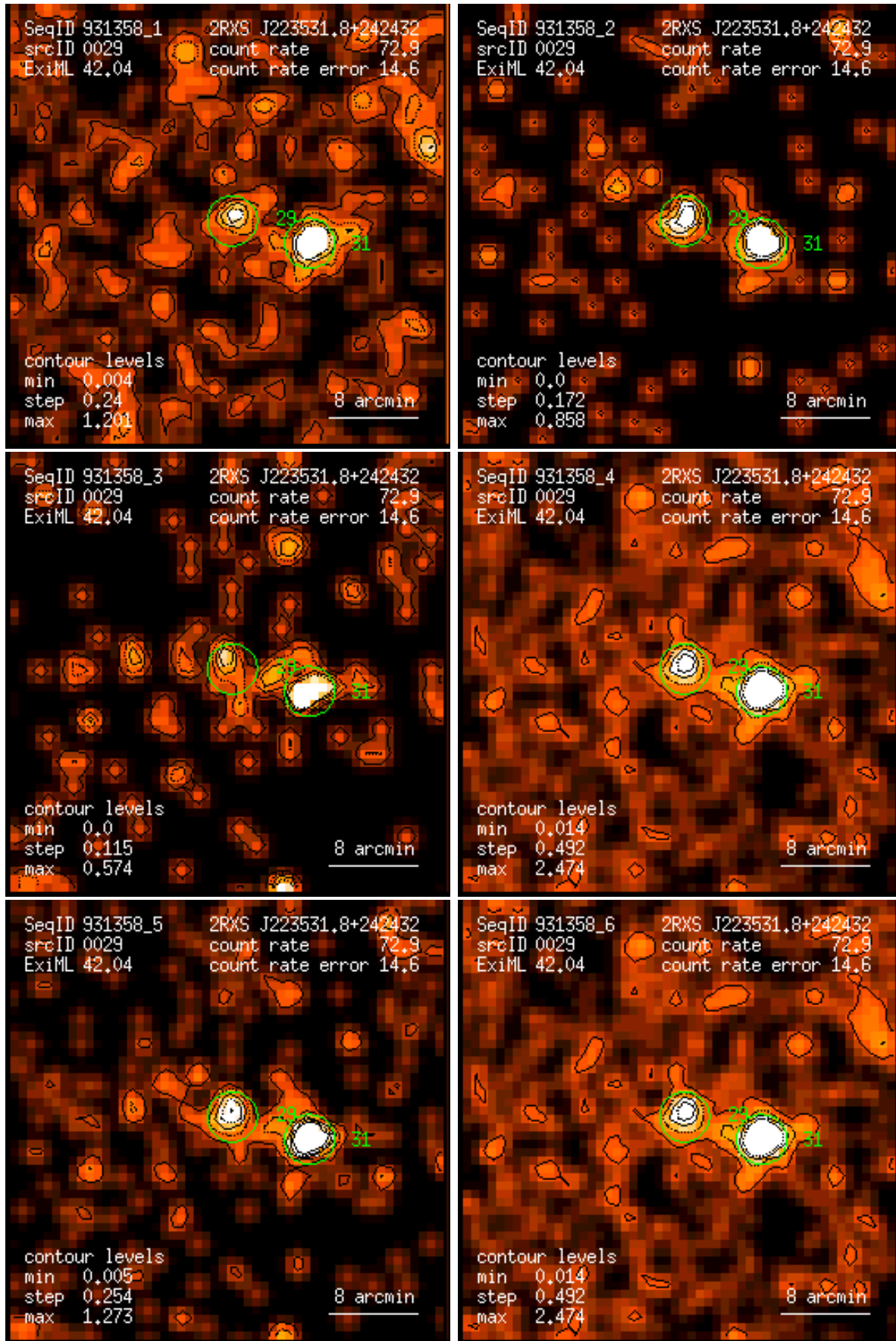
Figure 29: RASS 931358: detection 0029: band rate images, Gaussian filter: (1) PSPC channels 11 – 41, (2) 52 – 90, (3) 91 – 201, (4) 11 – 235, (5) 52 – 201, (6) 11 – 201. Broad band rates in counts/ks. Band rate contour levels in counts/ks/arcmin 2 .
