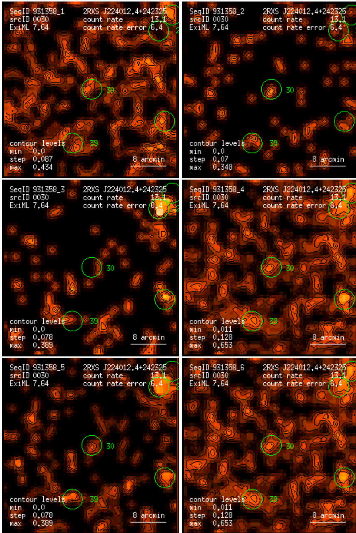
Figure 30: RASS 931358: detection 0030: band rate images, Gaussian filter: (1) PSPC channels 11 – 41, (2) 52 – 90, (3) 91 – 201, (4) 11 – 235, (5) 52 – 201, (6) 11 – 201. Broad band rates in counts/ks. Band rate contour levels in counts/ks/arcmin 2 .
