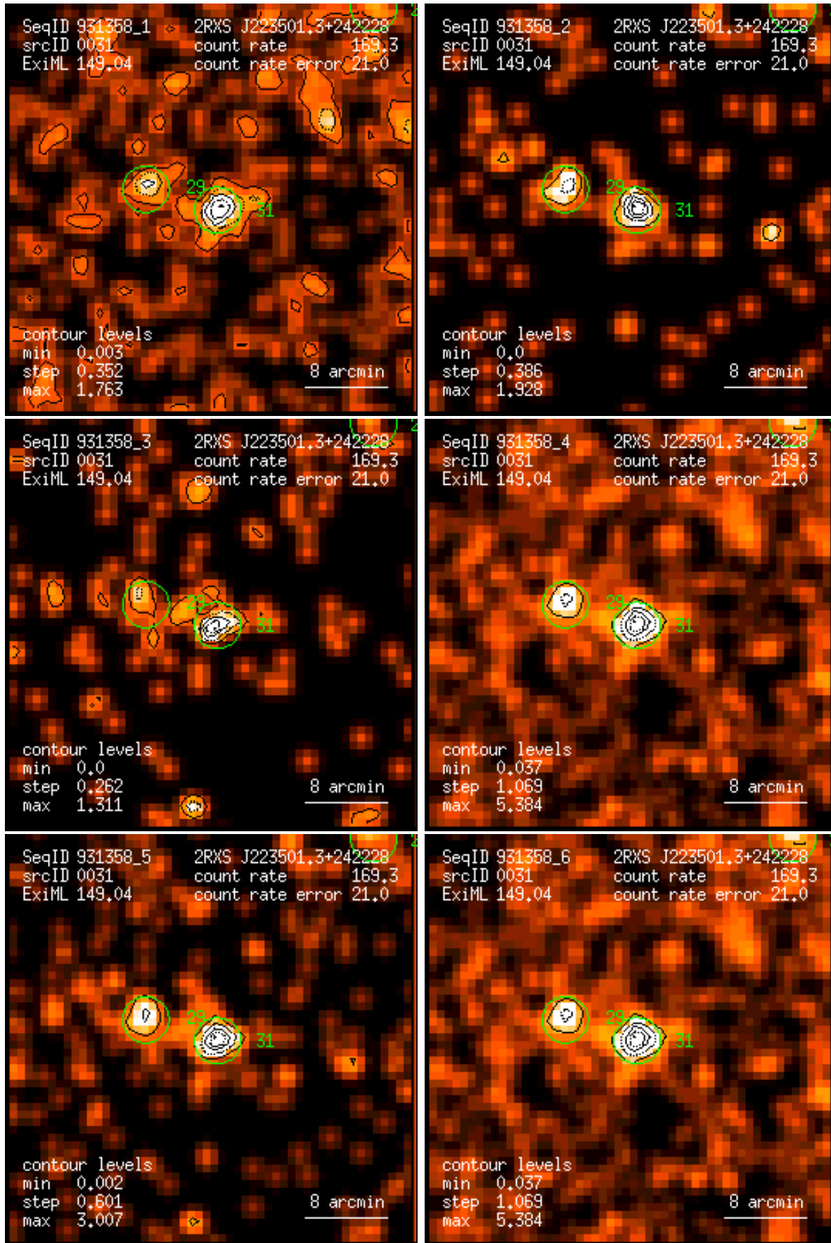
Figure 31: RASS 931358: detection 0031: band rate images, Gaussian filter: (1) PSPC channels 11 – 41, (2) 52 – 90, (3) 91 – 201, (4) 11 – 235, (5) 52 – 201, (6) 11 – 201. Broad band rates in counts/ks. Band rate contour levels in counts/ks/arcmin 2 .
