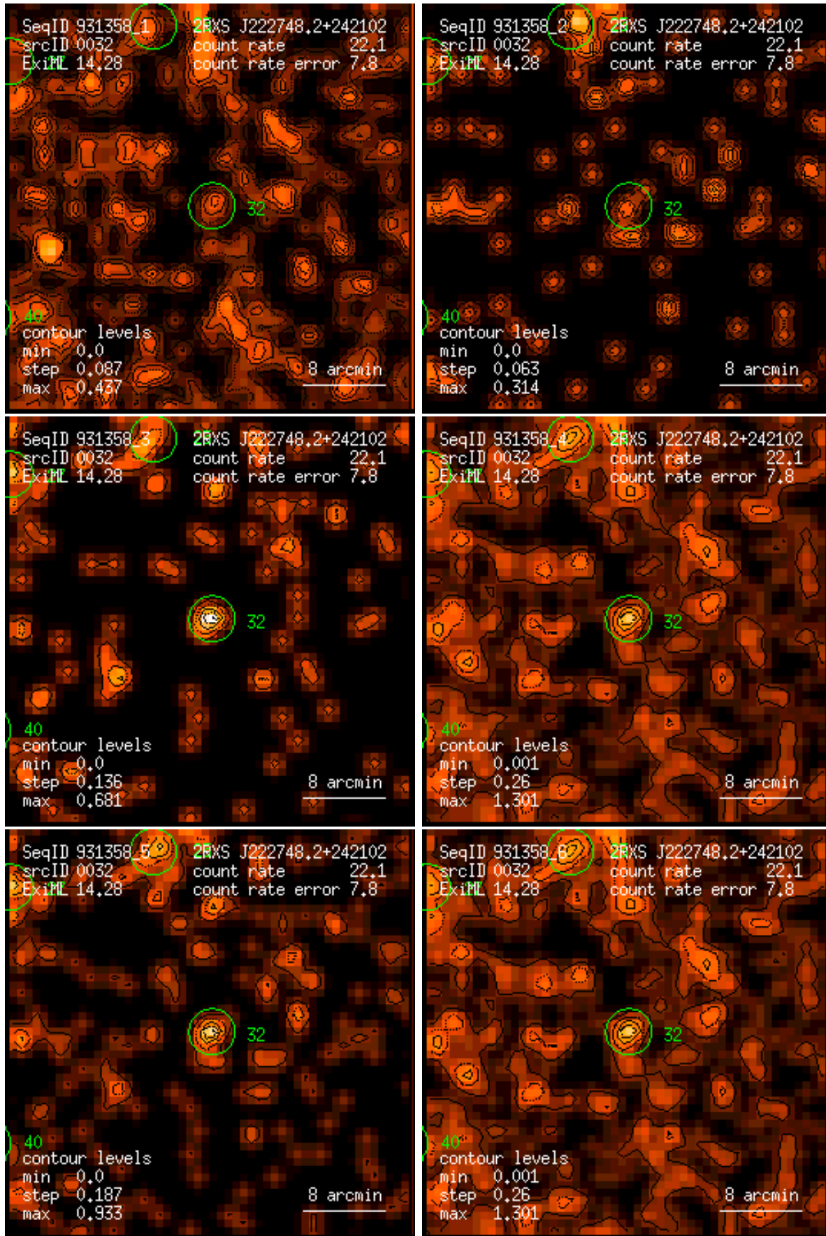
Figure 32: RASS 931358: detection 0032: band rate images, Gaussian filter: (1) PSPC channels 11 – 41, (2) 52 – 90, (3) 91 – 201, (4) 11 – 235, (5) 52 – 201, (6) 11 – 201. Broad band rates in counts/ks. Band rate contour levels in counts/ks/arcmin 2 .
