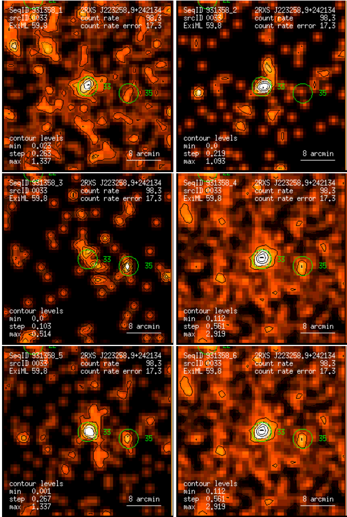
Figure 33: RASS 931358: detection 0033: band rate images, Gaussian filter: (1) PSPC channels 11 – 41, (2) 52 – 90, (3) 91 – 201, (4) 11 – 235, (5) 52 – 201, (6) 11 – 201. Broad band rates in counts/ks. Band rate contour levels in counts/ks/arcmin 2 .
