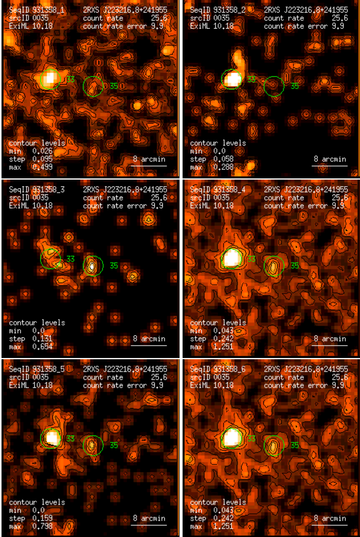
Figure 35: RASS 931358: detection 0035: band rate images, Gaussian filter: (1) PSPC channels 11 – 41, (2) 52 – 90, (3) 91 – 201, (4) 11 – 235, (5) 52 – 201, (6) 11 – 201. Broad band rates in counts/ks. Band rate contour levels in counts/ks/arcmin 2 .
