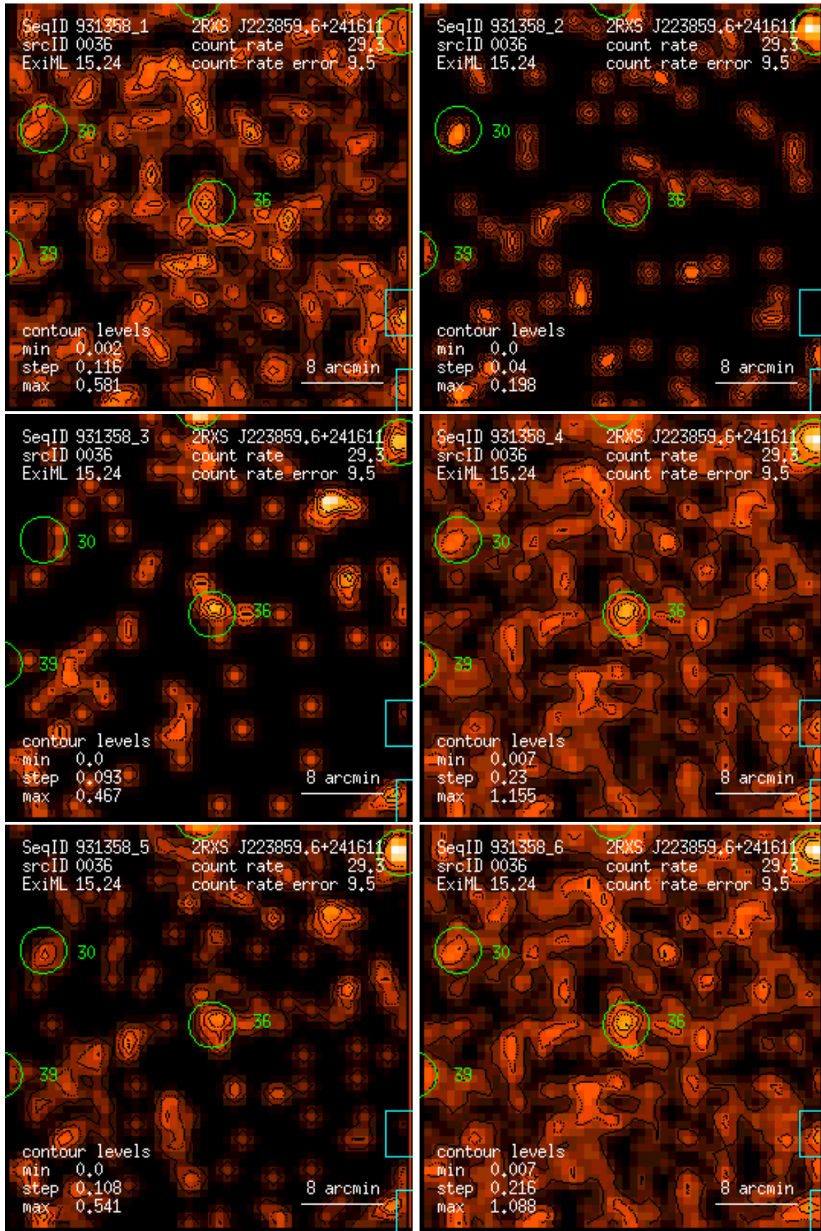
Figure 36: RASS 931358: detection 0036: band rate images, Gaussian filter: (1) PSPC channels 11 – 41, (2) 52 – 90, (3) 91 – 201, (4) 11 – 235, (5) 52 – 201, (6) 11 – 201. Broad band rates in counts/ks. Band rate contour levels in counts/ks/arcmin 2 .
