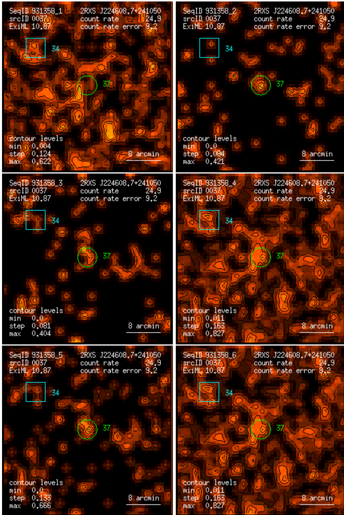
Figure 37: RASS 931358: detection 0037: band rate images, Gaussian filter: (1) PSPC channels 11 – 41, (2) 52 – 90, (3) 91 – 201, (4) 11 – 235, (5) 52 – 201, (6) 11 – 201. Broad band rates in counts/ks. Band rate contour levels in counts/ks/arcmin 2 .
