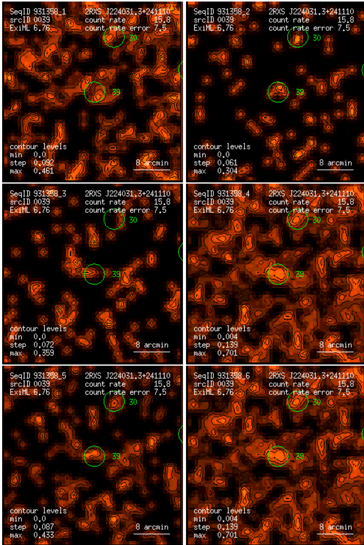
Figure 39: RASS 931358: detection 0039: band rate images, Gaussian filter: (1) PSPC channels 11 – 41, (2) 52 – 90, (3) 91 – 201, (4) 11 – 235, (5) 52 – 201, (6) 11 – 201. Broad band rates in counts/ks. Band rate contour levels in counts/ks/arcmin 2 .
