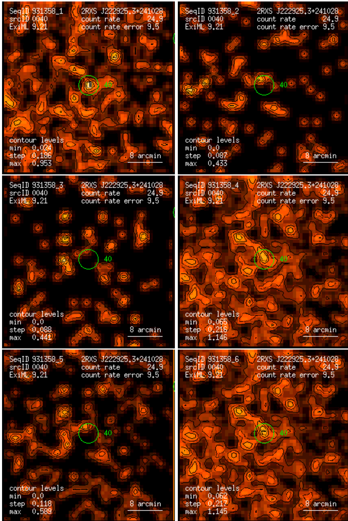
Figure 40: RASS 931358: detection 0040: band rate images, Gaussian filter: (1) PSPC channels 11 – 41, (2) 52 – 90, (3) 91 – 201, (4) 11 – 235, (5) 52 – 201, (6) 11 – 201. Broad band rates in counts/ks. Band rate contour levels in counts/ks/arcmin 2 .
