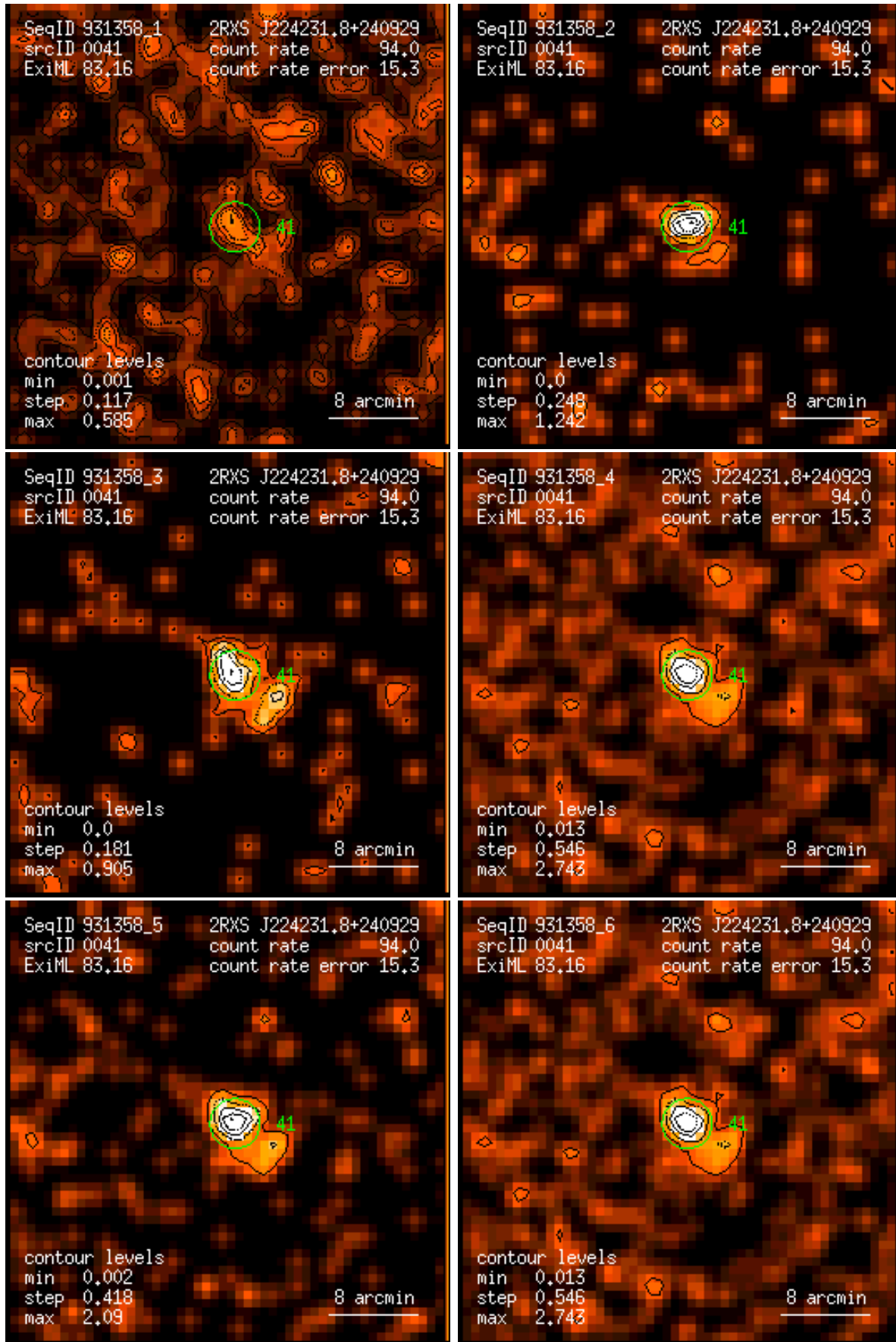
Figure 41: RASS 931358: detection 0041: band rate images, Gaussian filter: (1) PSPC channels 11 – 41, (2) 52 – 90, (3) 91 – 201, (4) 11 – 235, (5) 52 – 201, (6) 11 – 201. Broad band rates in counts/ks. Band rate contour levels in counts/ks/arcmin 2 .
