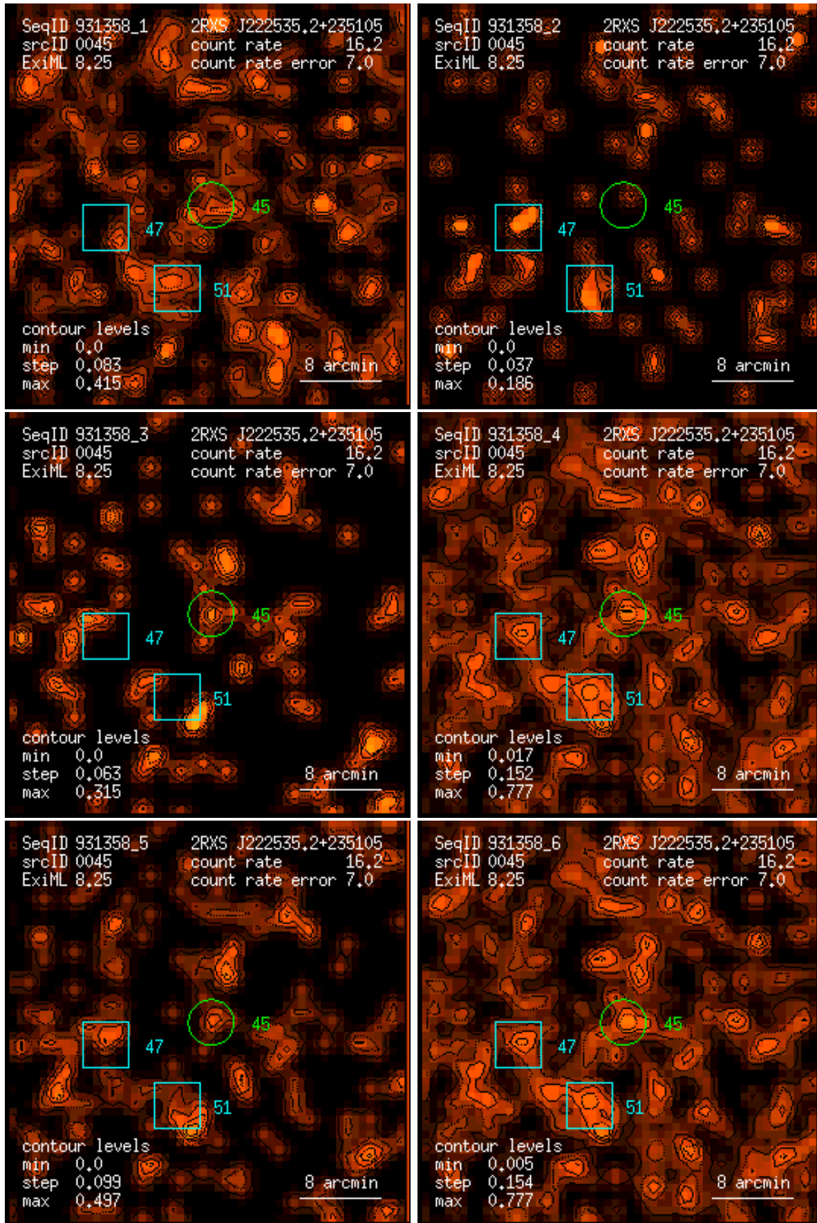
Figure 45: RASS 931358: detection 0045: band rate images, Gaussian filter: (1) PSPC channels 11 – 41, (2) 52 – 90, (3) 91 – 201, (4) 11 – 235, (5) 52 – 201, (6) 11 – 201. Broad band rates in counts/ks. Band rate contour levels in counts/ks/arcmin 2 .
