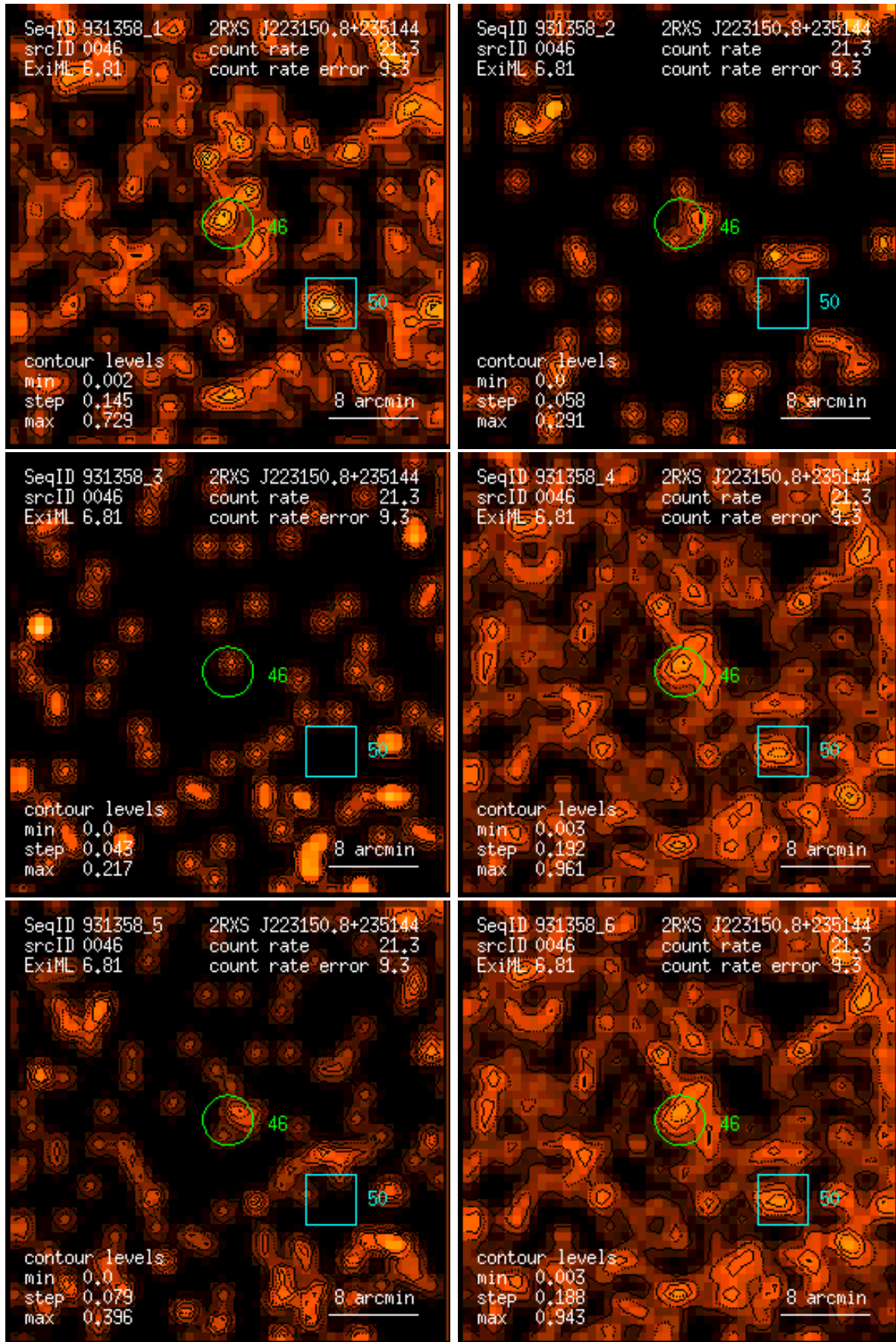
Figure 46: RASS 931358: detection 0046: band rate images, Gaussian filter: (1) PSPC channels 11 – 41, (2) 52 – 90, (3) 91 – 201, (4) 11 – 235, (5) 52 – 201, (6) 11 – 201. Broad band rates in counts/ks. Band rate contour levels in counts/ks/arcmin 2 .
