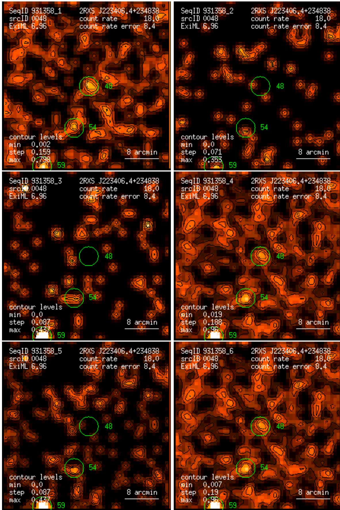
Figure 48: RASS 931358: detection 0048: band rate images, Gaussian filter: (1) PSPC channels 11 – 41, (2) 52 – 90, (3) 91 – 201, (4) 11 – 235, (5) 52 – 201, (6) 11 – 201. Broad band rates in counts/ks. Band rate contour levels in counts/ks/arcmin 2 .
