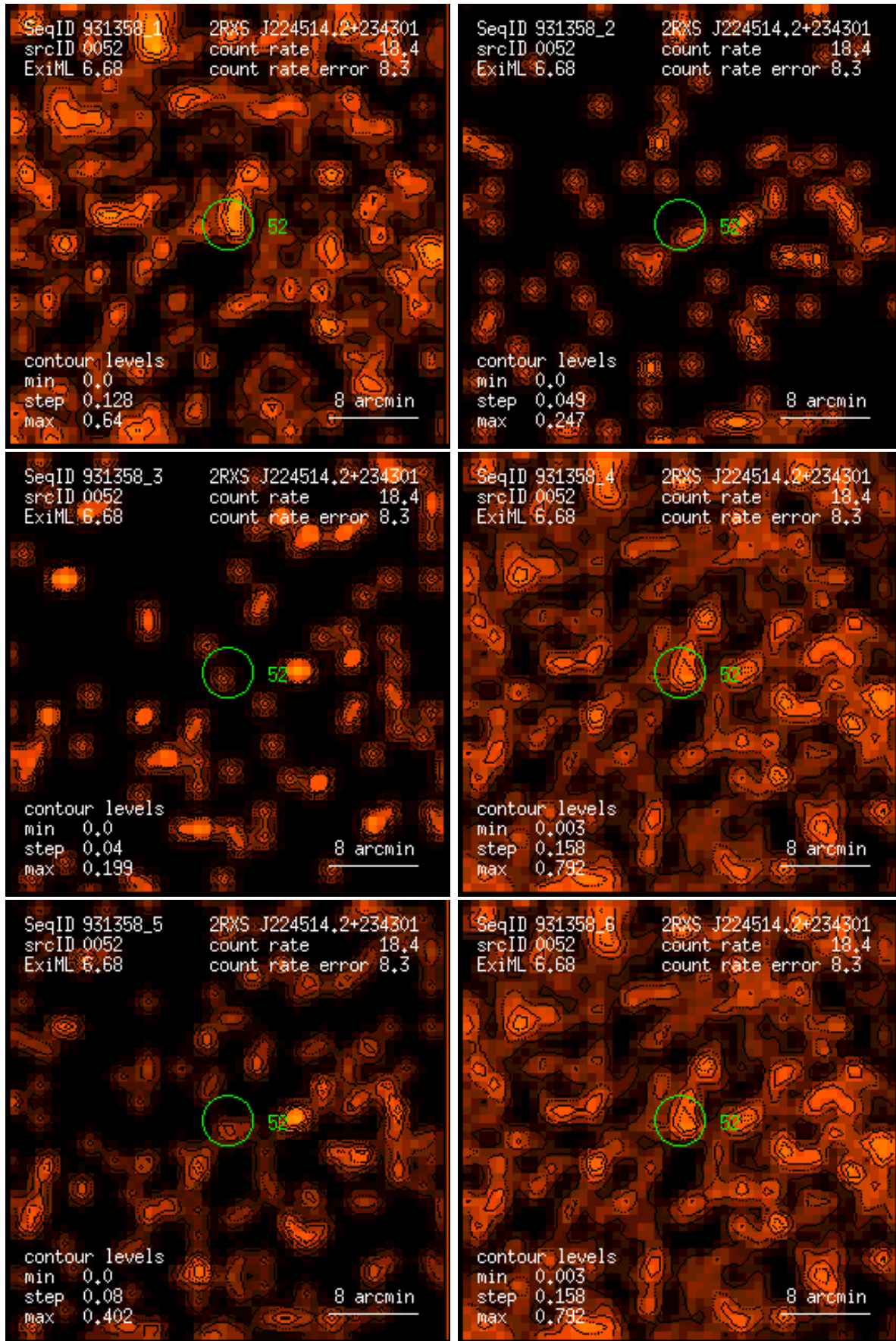
Figure 52: RASS 931358: detection 0052: band rate images, Gaussian filter: (1) PSPC channels 11 – 41, (2) 52 – 90, (3) 91 – 201, (4) 11 – 235, (5) 52 – 201, (6) 11 – 201. Broad band rates in counts/ks. Band rate contour levels in counts/ks/arcmin 2 .
