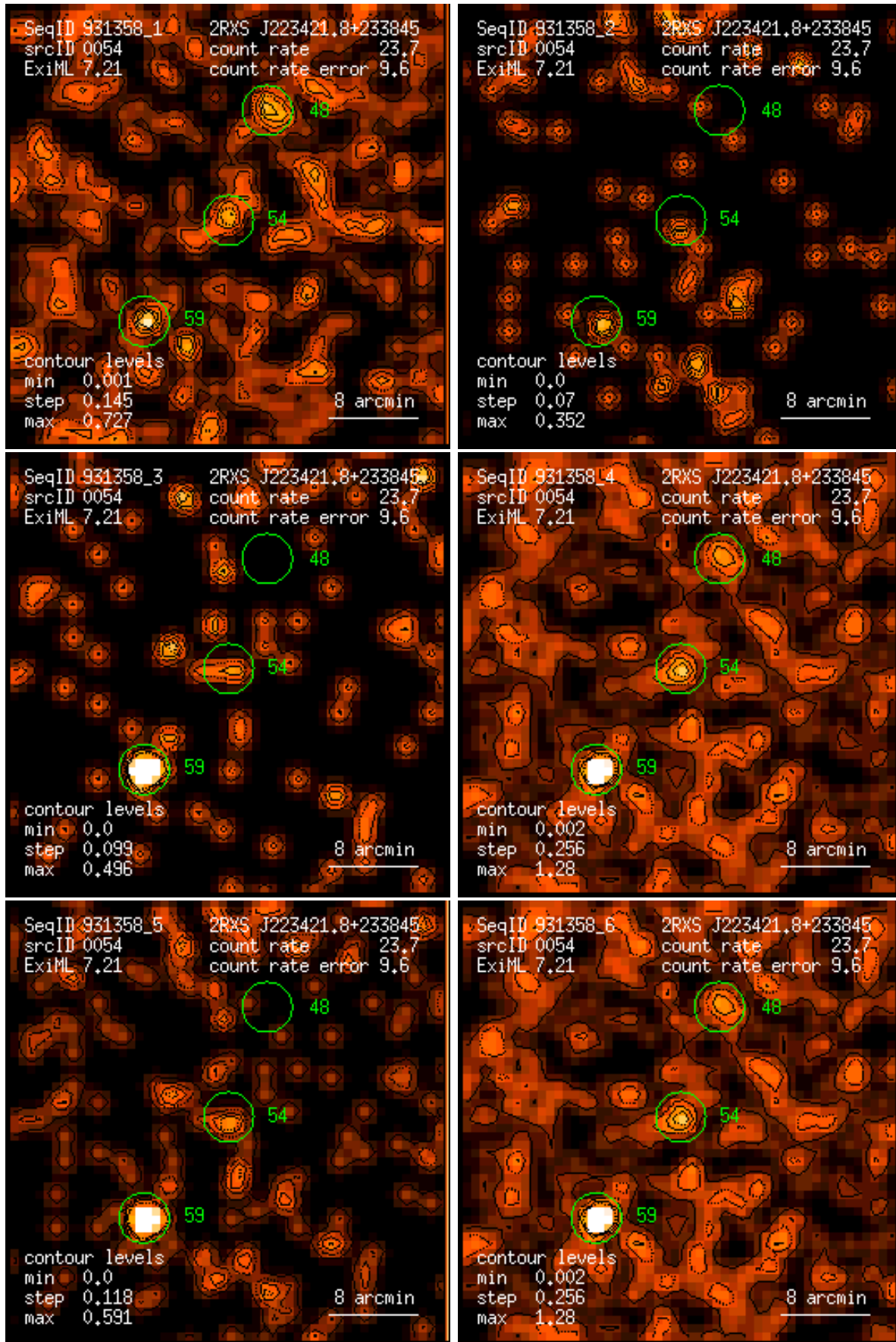
Figure 54: RASS 931358: detection 0054: band rate images, Gaussian filter: (1) PSPC channels 11 – 41, (2) 52 – 90, (3) 91 – 201, (4) 11 – 235, (5) 52 – 201, (6) 11 – 201. Broad band rates in counts/ks. Band rate contour levels in counts/ks/arcmin 2 .
