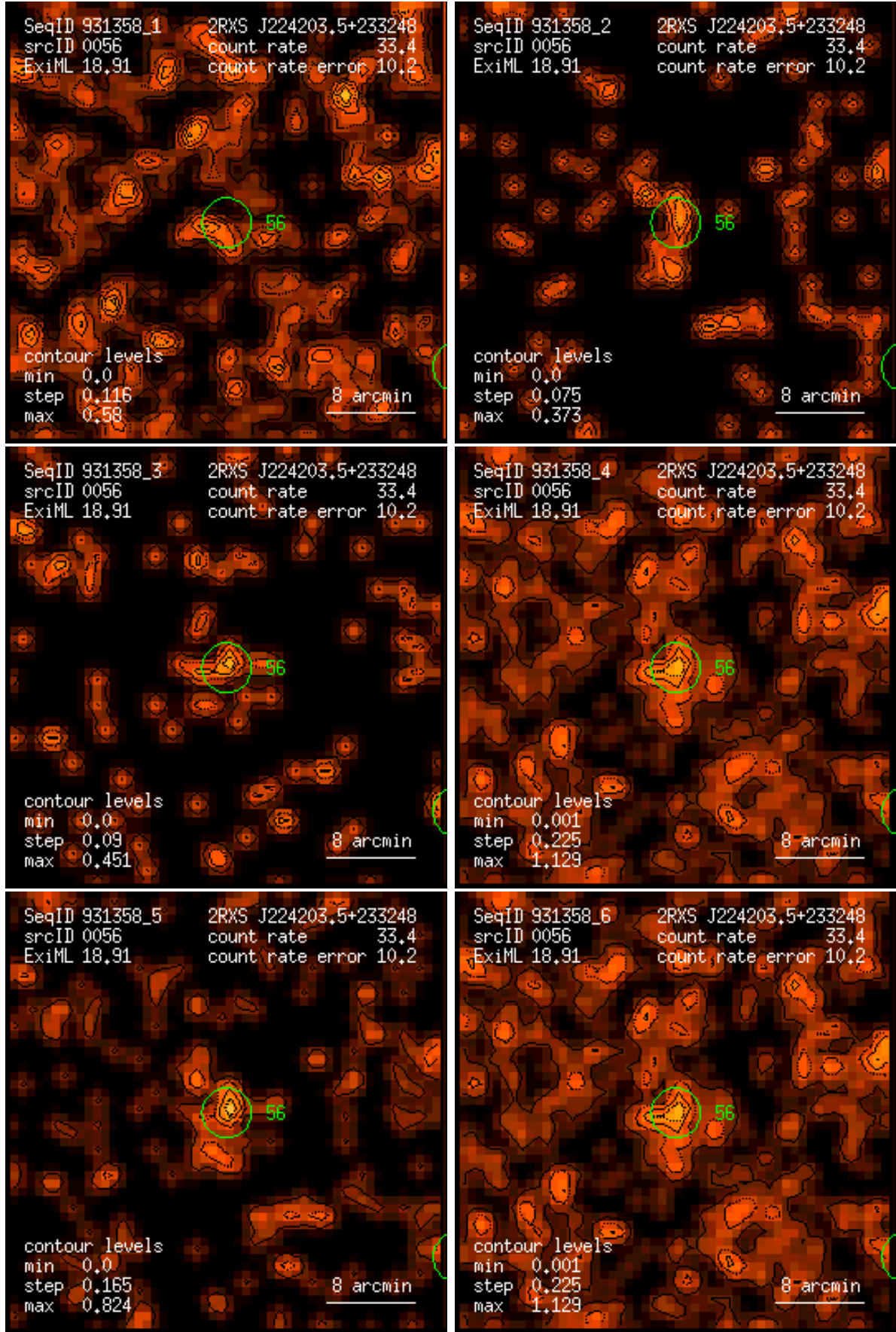
Figure 56: RASS 931358: detection 0056: band rate images, Gaussian filter: (1) PSPC channels 11 – 41, (2) 52 – 90, (3) 91 – 201, (4) 11 – 235, (5) 52 – 201, (6) 11 – 201. Broad band rates in counts/ks. Band rate contour levels in counts/ks/arcmin 2 .
