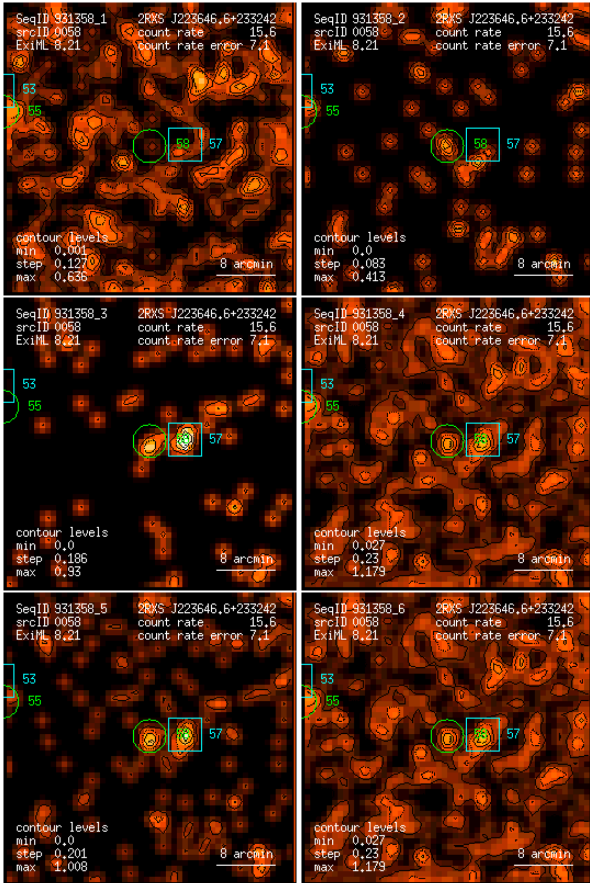
Figure 58: RASS 931358: detection 0058: band rate images, Gaussian filter: (1) PSPC channels 11 – 41, (2) 52 – 90, (3) 91 – 201, (4) 11 – 235, (5) 52 – 201, (6) 11 – 201. Broad band rates in counts/ks. Band rate contour levels in counts/ks/arcmin 2 .
