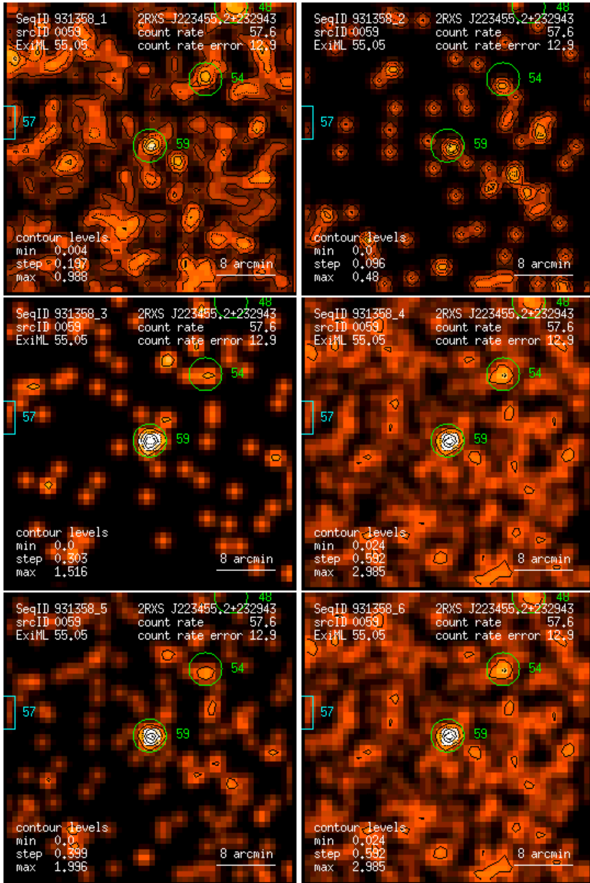
Figure 59: RASS 931358: detection 0059: band rate images, Gaussian filter: (1) PSPC channels 11 – 41, (2) 52 – 90, (3) 91 – 201, (4) 11 – 235, (5) 52 – 201, (6) 11 – 201. Broad band rates in counts/ks. Band rate contour levels in counts/ks/arcmin 2 .
