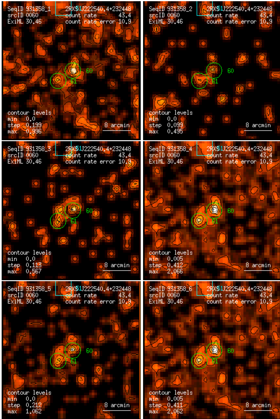
Figure 60: RASS 931358: detection 0060: band rate images, Gaussian filter: (1) PSPC channels 11 – 41, (2) 52 – 90, (3) 91 – 201, (4) 11 – 235, (5) 52 – 201, (6) 11 – 201. Broad band rates in counts/ks. Band rate contour levels in counts/ks/arcmin 2 .
