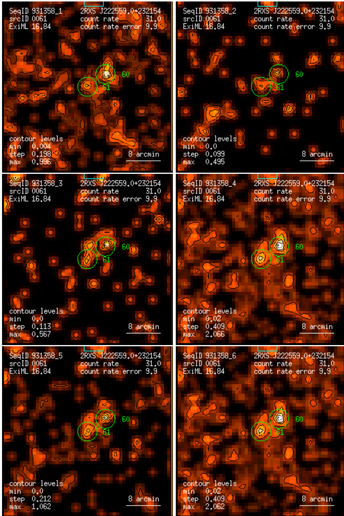
Figure 61: RASS 931358: detection 0061: band rate images, Gaussian filter: (1) PSPC channels 11 – 41, (2) 52 – 90, (3) 91 – 201, (4) 11 – 235, (5) 52 – 201, (6) 11 – 201. Broad band rates in counts/ks. Band rate contour levels in counts/ks/arcmin 2 .
