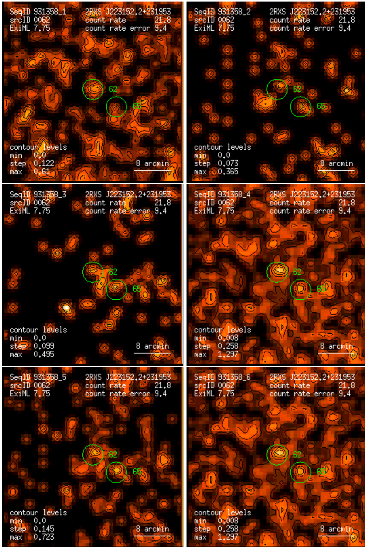
Figure 62: RASS 931358: detection 0062: band rate images, Gaussian filter: (1) PSPC channels 11 – 41, (2) 52 – 90, (3) 91 – 201, (4) 11 – 235, (5) 52 – 201, (6) 11 – 201. Broad band rates in counts/ks. Band rate contour levels in counts/ks/arcmin 2 .
