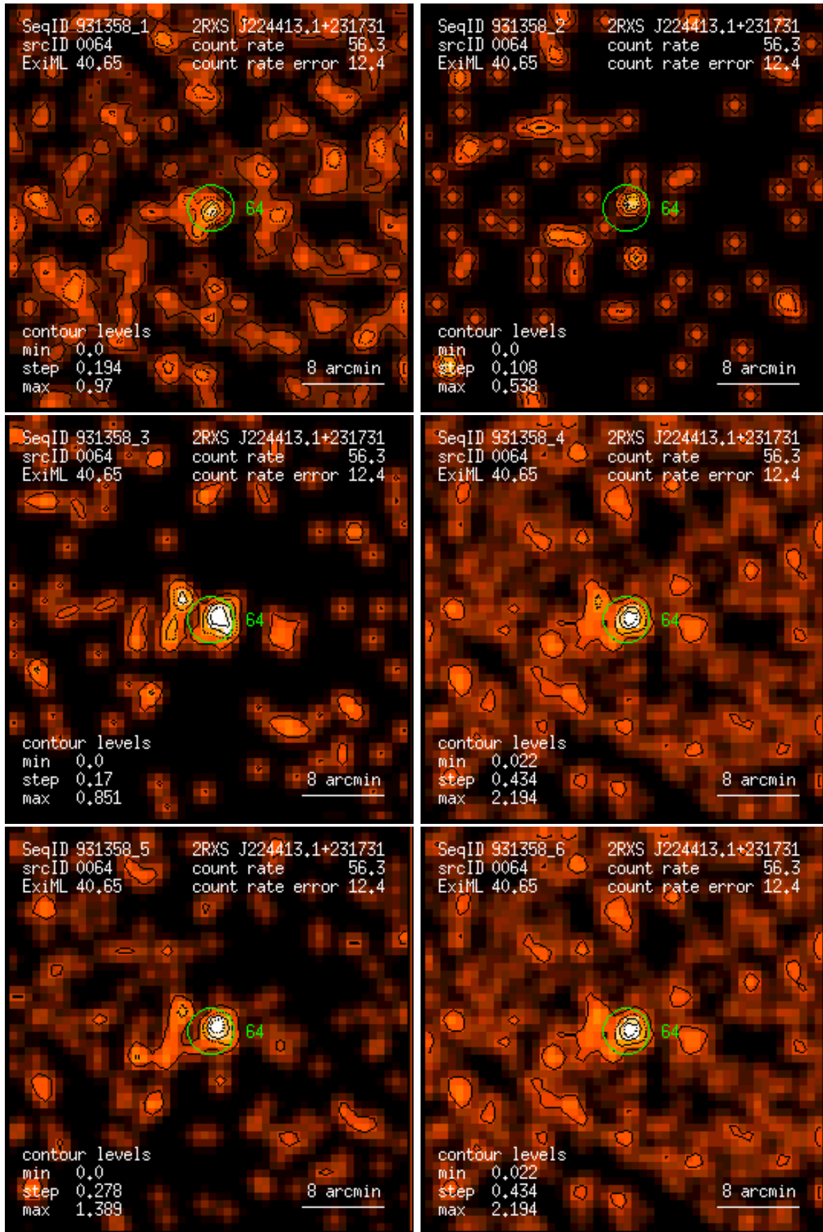
Figure 64: RASS 931358: detection 0064: band rate images, Gaussian filter: (1) PSPC channels 11 – 41, (2) 52 – 90, (3) 91 – 201, (4) 11 – 235, (5) 52 – 201, (6) 11 – 201. Broad band rates in counts/ks. Band rate contour levels in counts/ks/arcmin 2 .
