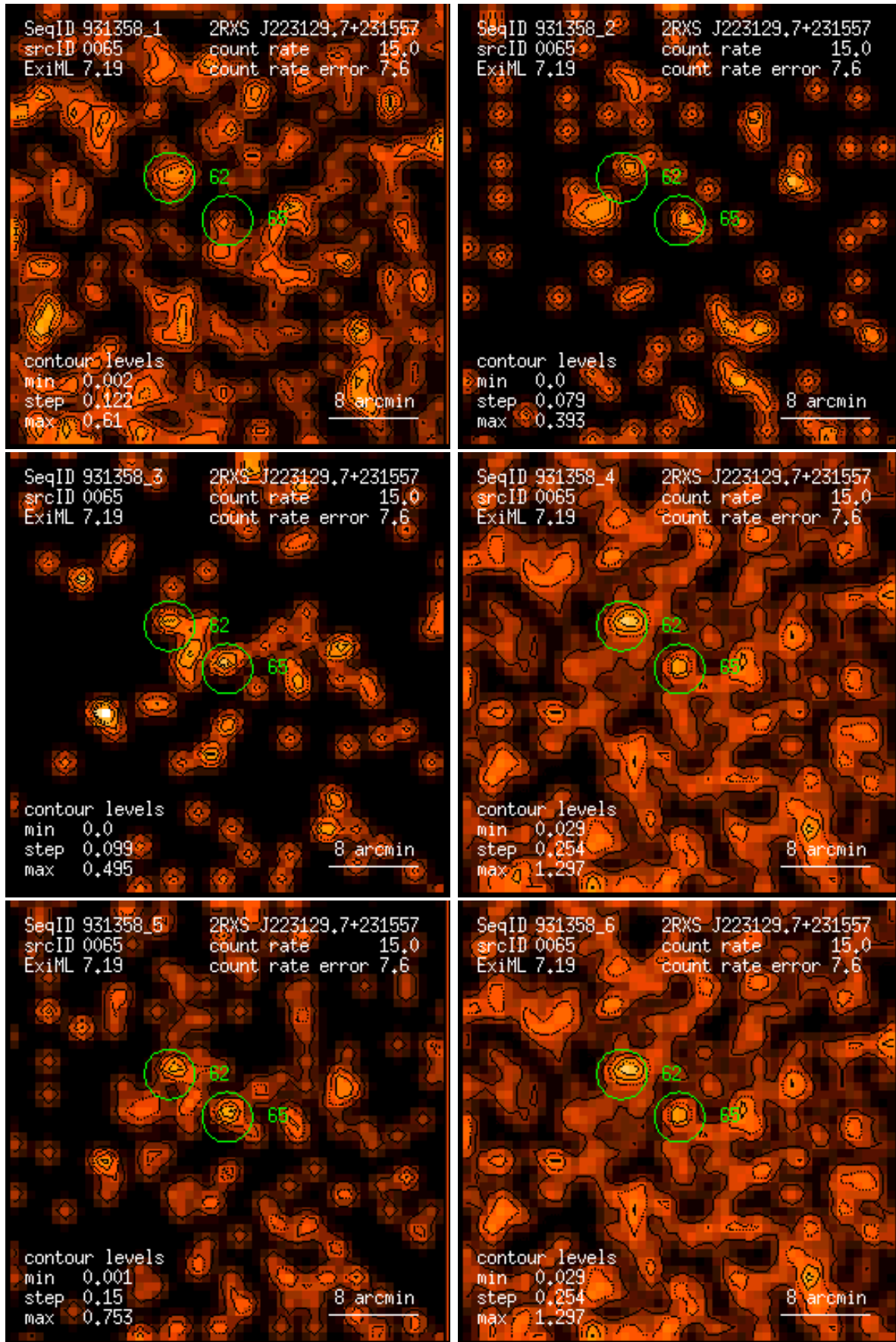
Figure 65: RASS 931358: detection 0065: band rate images, Gaussian filter: (1) PSPC channels 11 – 41, (2) 52 – 90, (3) 91 – 201, (4) 11 – 235, (5) 52 – 201, (6) 11 – 201. Broad band rates in counts/ks. Band rate contour levels in counts/ks/arcmin 2 .
