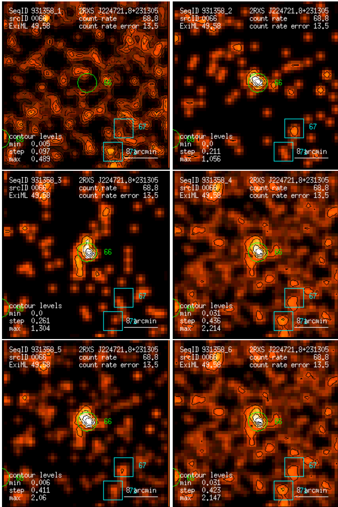
Figure 66: RASS 931358: detection 0066: band rate images, Gaussian filter: (1) PSPC channels 11 – 41, (2) 52 – 90, (3) 91 – 201, (4) 11 – 235, (5) 52 – 201, (6) 11 – 201. Broad band rates in counts/ks. Band rate contour levels in counts/ks/arcmin 2 .
