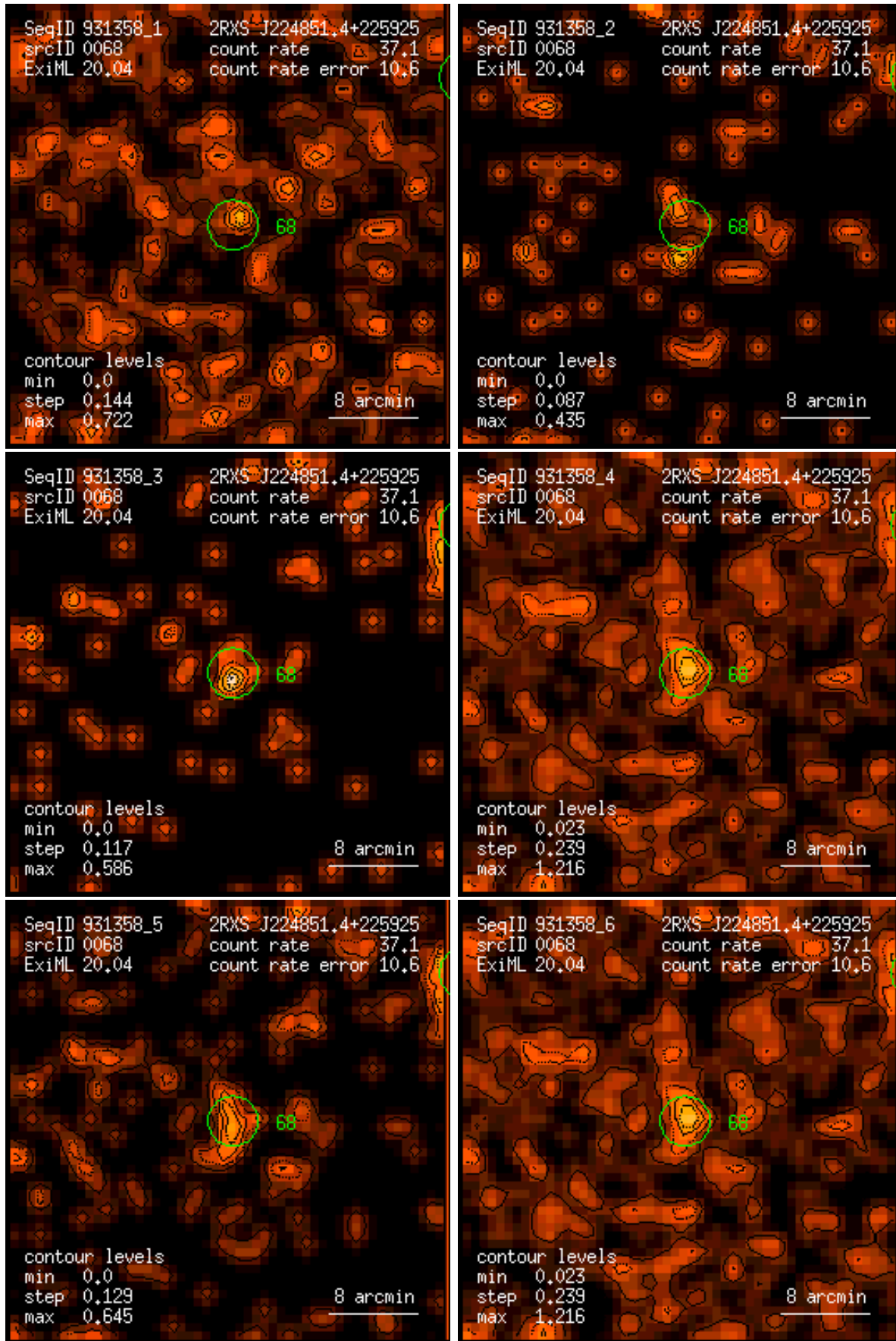
Figure 68: RASS 931358: detection 0068: band rate images, Gaussian filter: (1) PSPC channels 11 – 41, (2) 52 – 90, (3) 91 – 201, (4) 11 – 235, (5) 52 – 201, (6) 11 – 201. Broad band rates in counts/ks. Band rate contour levels in counts/ks/arcmin 2 .
