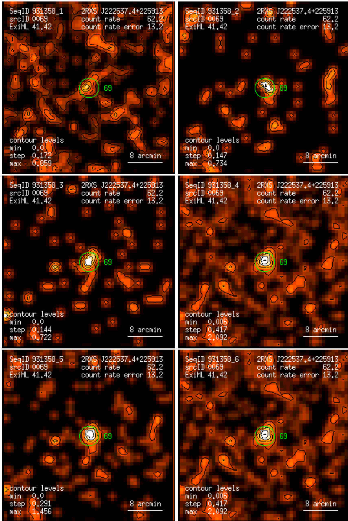
Figure 69: RASS 931358: detection 0069: band rate images, Gaussian filter: (1) PSPC channels 11 – 41, (2) 52 – 90, (3) 91 – 201, (4) 11 – 235, (5) 52 – 201, (6) 11 – 201. Broad band rates in counts/ks. Band rate contour levels in counts/ks/arcmin 2 .
