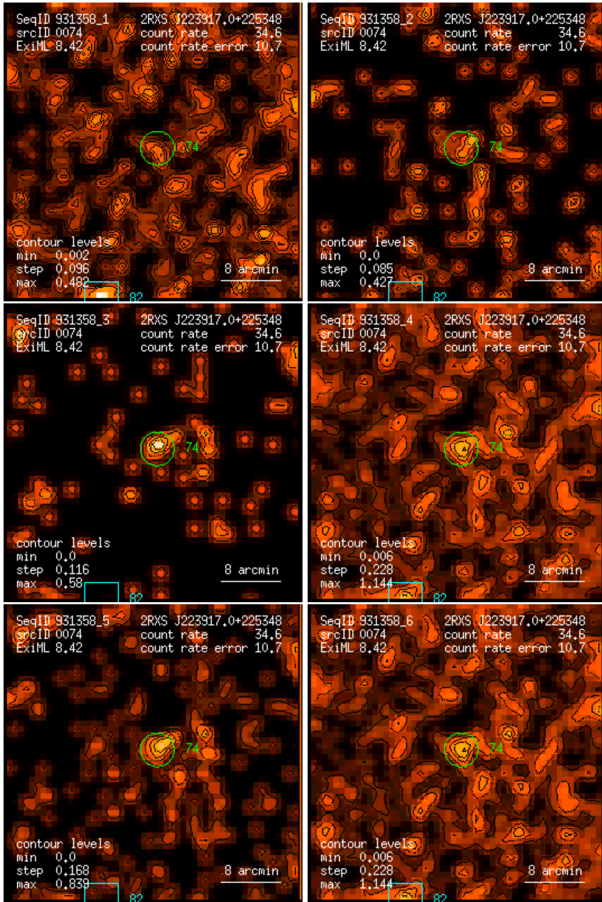
Figure 74: RASS 931358: detection 0074: band rate images, Gaussian filter: (1) PSPC channels 11 – 41, (2) 52 – 90, (3) 91 – 201, (4) 11 – 235, (5) 52 – 201, (6) 11 – 201. Broad band rates in counts/ks. Band rate contour levels in counts/ks/arcmin 2 .
