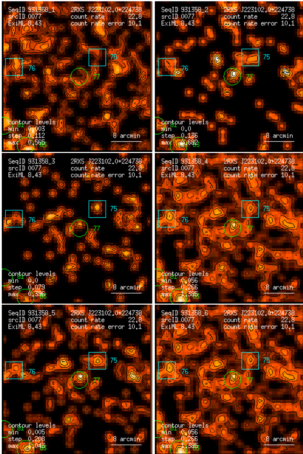
Figure 77: RASS 931358: detection 0077: band rate images, Gaussian filter: (1) PSPC channels 11 – 41, (2) 52 – 90, (3) 91 – 201, (4) 11 – 235, (5) 52 – 201, (6) 11 – 201. Broad band rates in counts/ks. Band rate contour levels in counts/ks/arcmin 2 .
