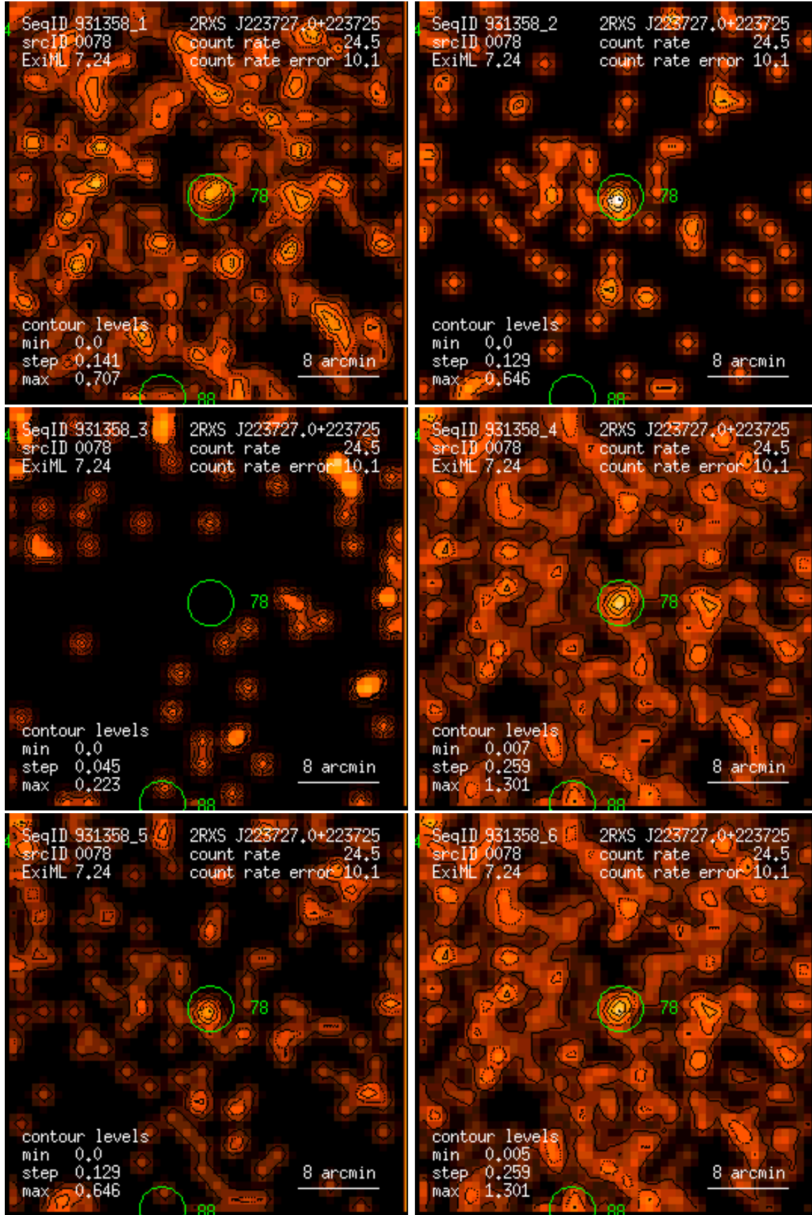
Figure 78: RASS 931358: detection 0078: band rate images, Gaussian filter: (1) PSPC channels 11 – 41, (2) 52 – 90, (3) 91 – 201, (4) 11 – 235, (5) 52 – 201, (6) 11 – 201. Broad band rates in counts/ks. Band rate contour levels in counts/ks/arcmin 2 .
