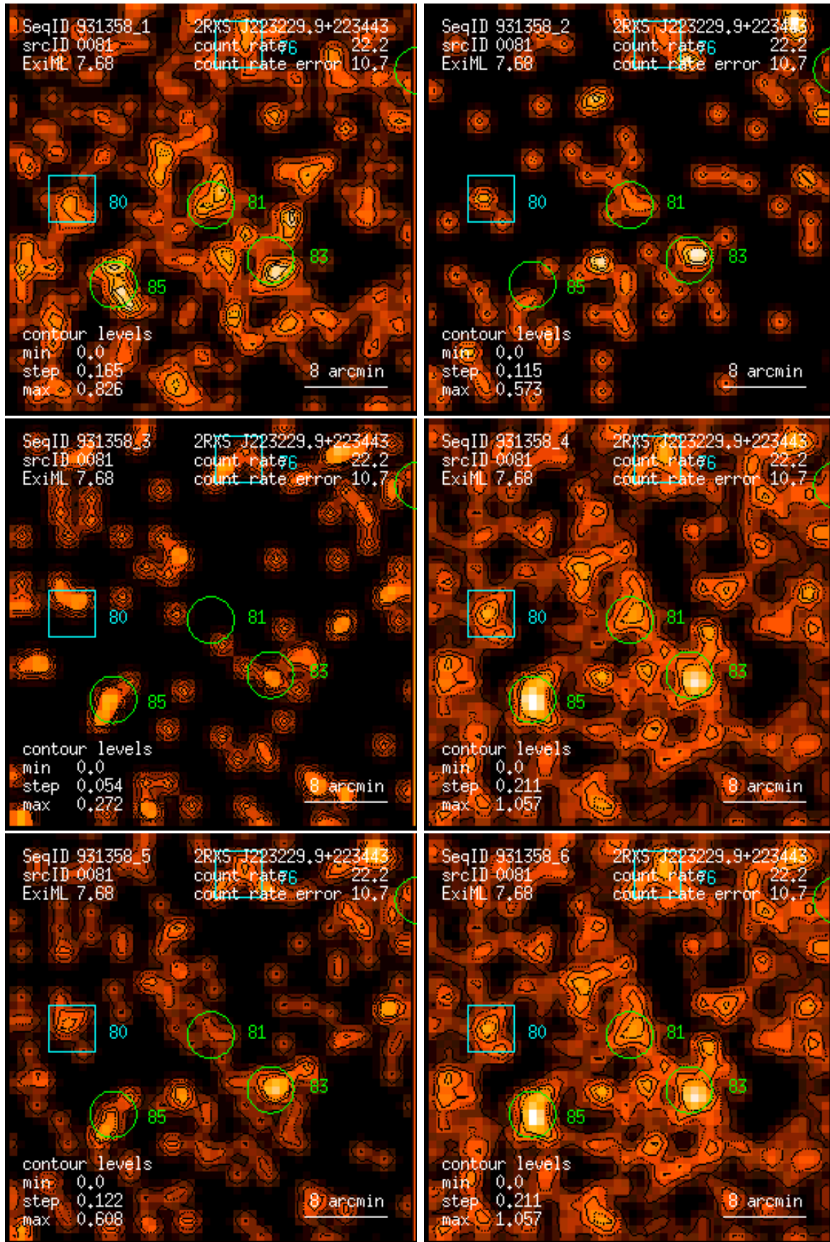
Figure 81: RASS 931358: detection 0081: band rate images, Gaussian filter: (1) PSPC channels 11 – 41, (2) 52 – 90, (3) 91 – 201, (4) 11 – 235, (5) 52 – 201, (6) 11 – 201. Broad band rates in counts/ks. Band rate contour levels in counts/ks/arcmin 2 .
