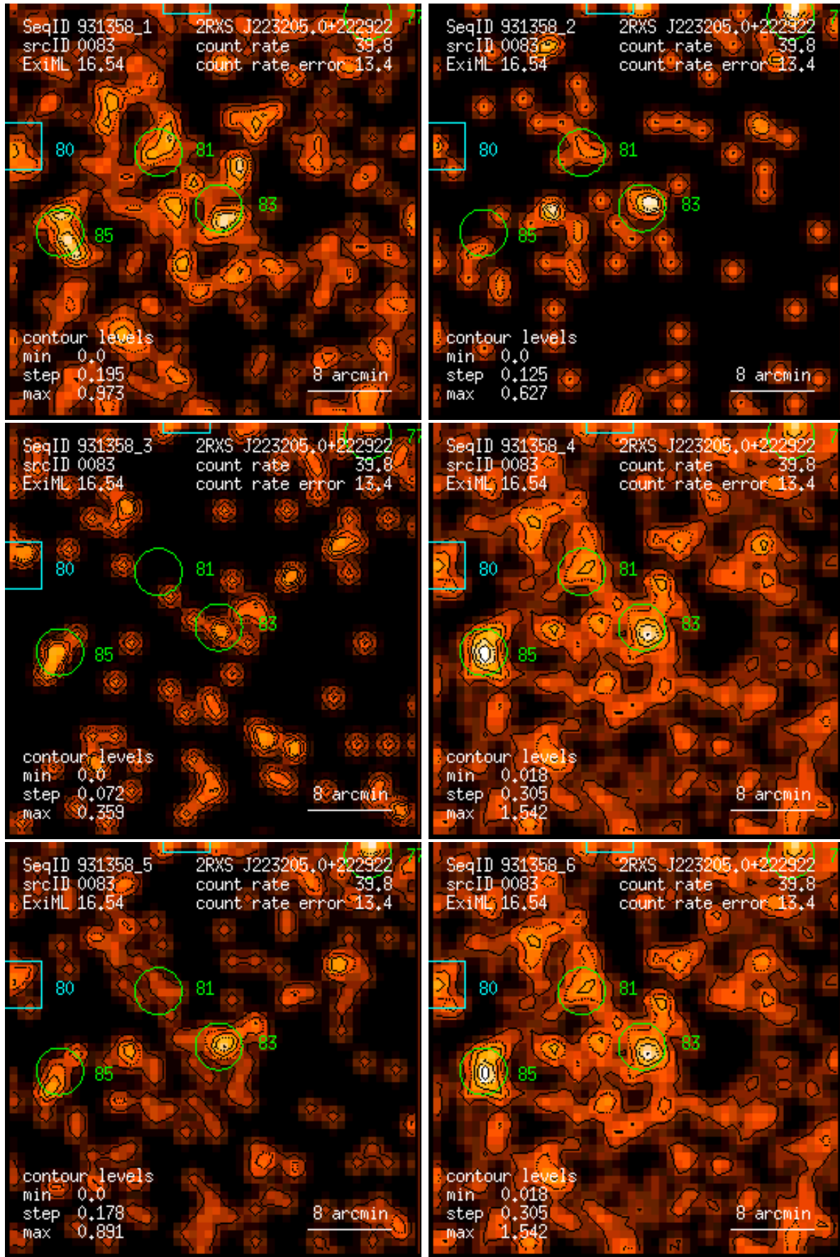
Figure 83: RASS 931358: detection 0083: band rate images, Gaussian filter: (1) PSPC channels 11 – 41, (2) 52 – 90, (3) 91 – 201, (4) 11 – 235, (5) 52 – 201, (6) 11 – 201. Broad band rates in counts/ks. Band rate contour levels in counts/ks/arcmin 2 .
