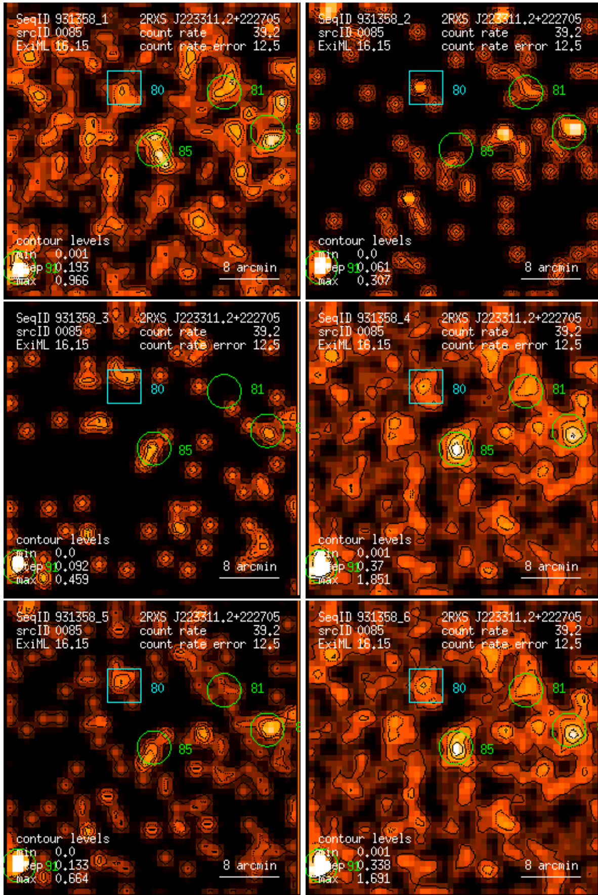
Figure 85: RASS 931358: detection 0085: band rate images, Gaussian filter: (1) PSPC channels 11 – 41, (2) 52 – 90, (3) 91 – 201, (4) 11 – 235, (5) 52 – 201, (6) 11 – 201. Broad band rates in counts/ks. Band rate contour levels in counts/ks/arcmin 2 .
