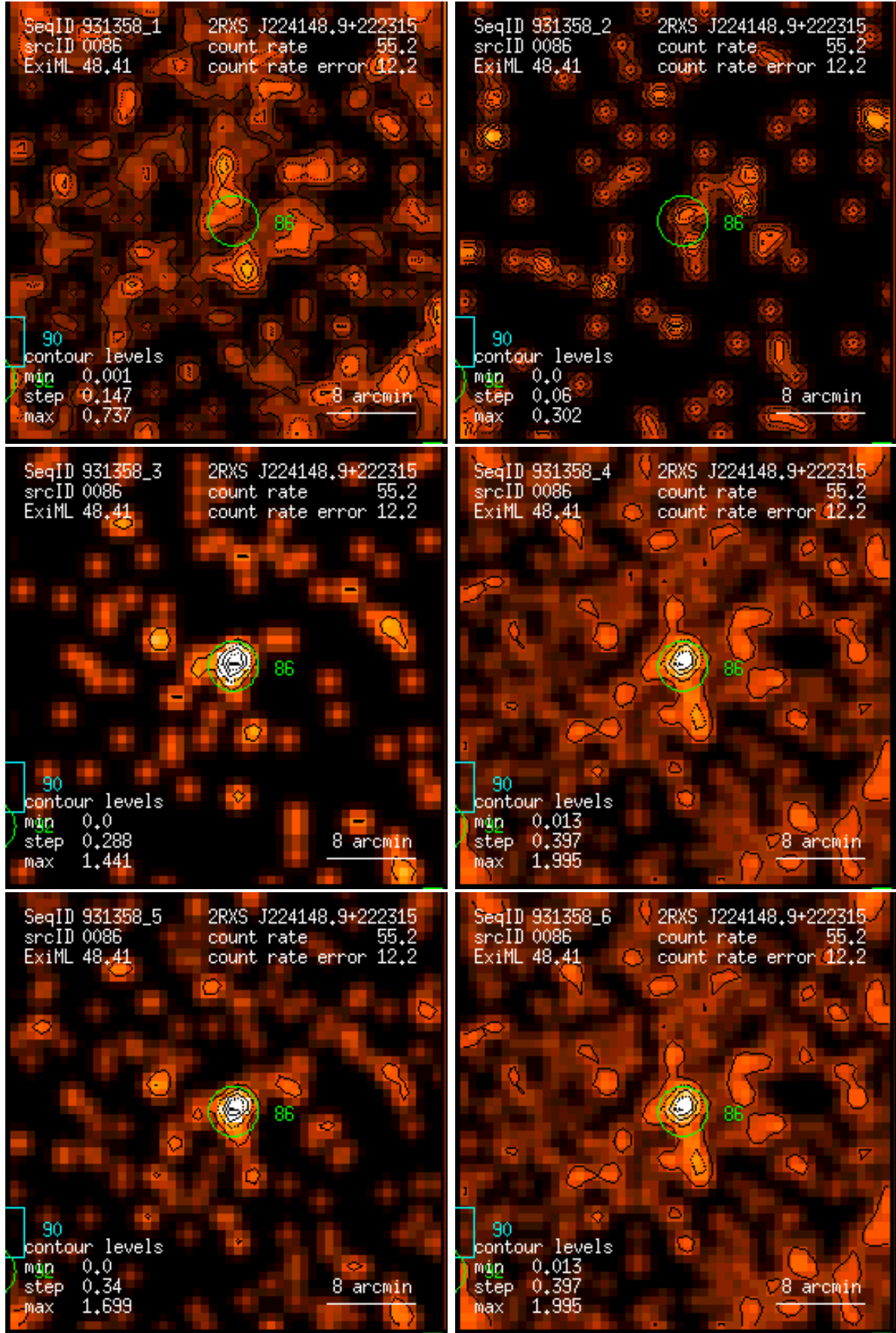
Figure 86: RASS 931358: detection 0086: band rate images, Gaussian filter: (1) PSPC channels 11 – 41, (2) 52 – 90, (3) 91 – 201, (4) 11 – 235, (5) 52 – 201, (6) 11 – 201. Broad band rates in counts/ks. Band rate contour levels in counts/ks/arcmin 2 .
