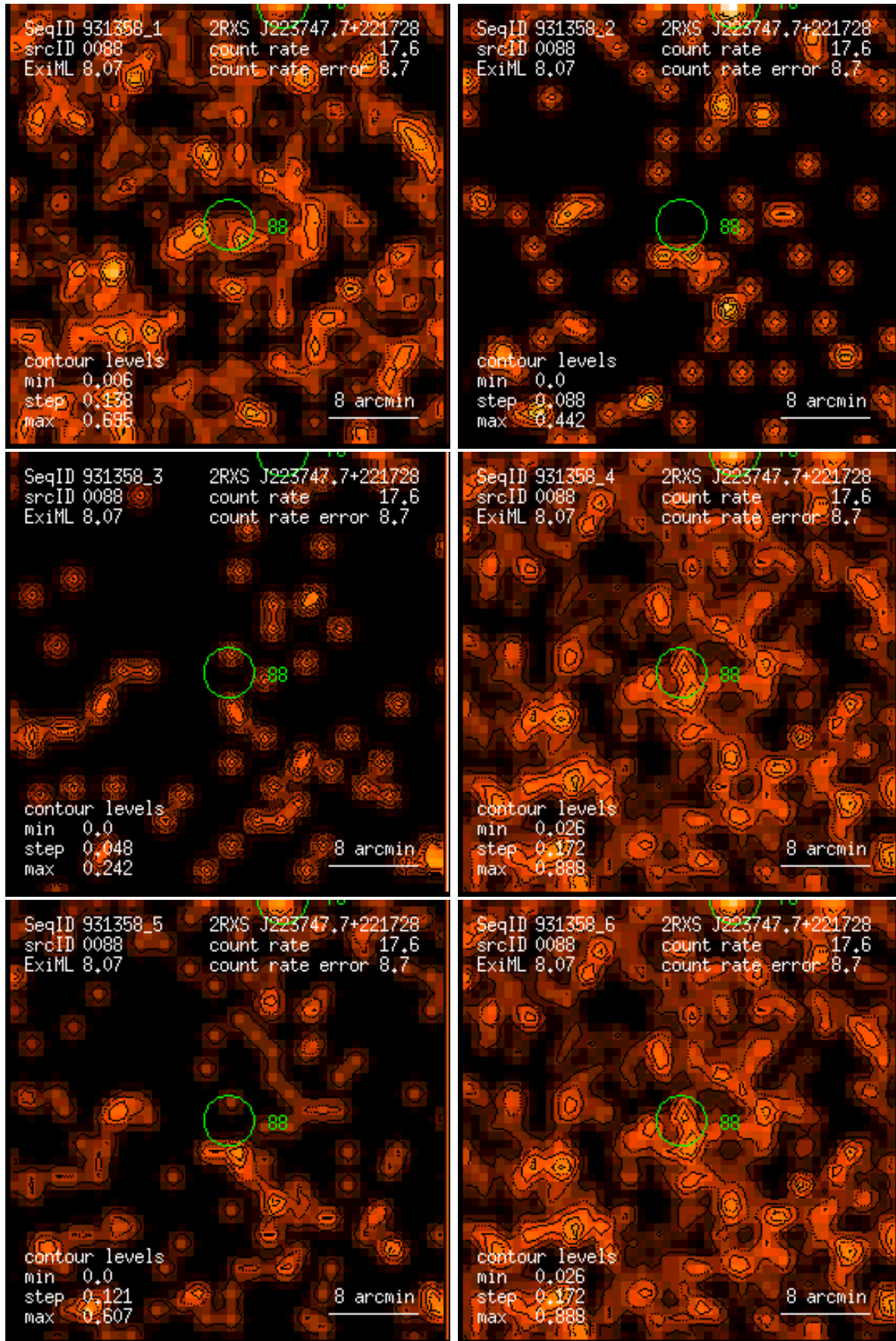
Figure 88: RASS 931358: detection 0088: band rate images, Gaussian filter: (1) PSPC channels 11 – 41, (2) 52 – 90, (3) 91 – 201, (4) 11 – 235, (5) 52 – 201, (6) 11 – 201. Broad band rates in counts/ks. Band rate contour levels in counts/ks/arcmin 2 .
