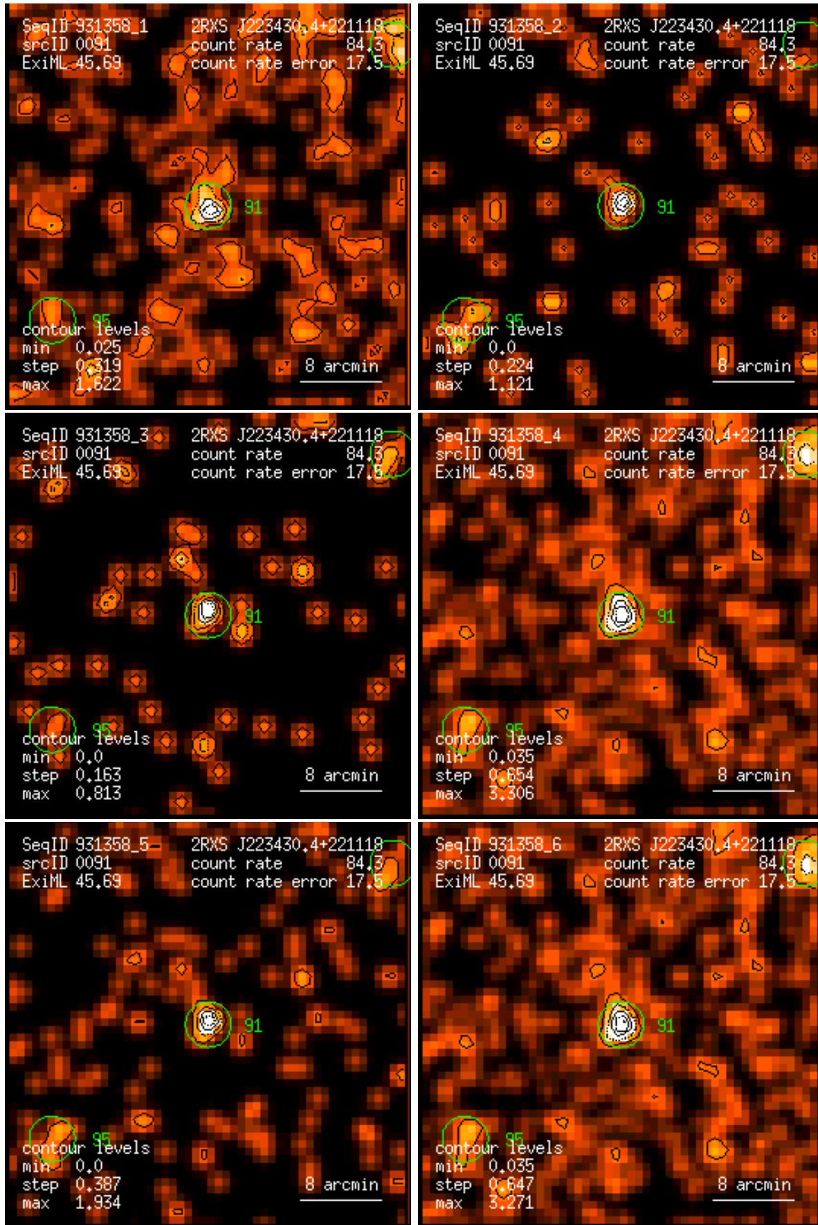
Figure 91: RASS 931358: detection 0091: band rate images, Gaussian filter: (1) PSPC channels 11 – 41, (2) 52 – 90, (3) 91 – 201, (4) 11 – 235, (5) 52 – 201, (6) 11 – 201. Broad band rates in counts/ks. Band rate contour levels in counts/ks/arcmin 2 .
