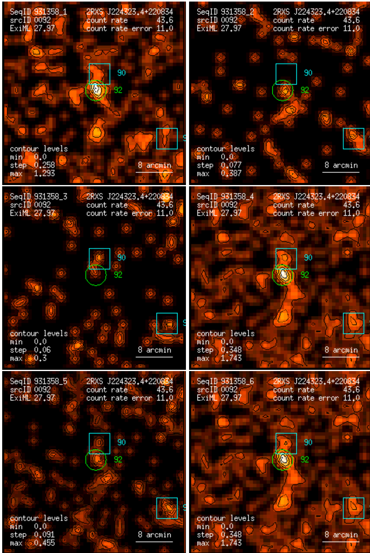
Figure 92: RASS 931358: detection 0092: band rate images, Gaussian filter: (1) PSPC channels 11 – 41, (2) 52 – 90, (3) 91 – 201, (4) 11 – 235, (5) 52 – 201, (6) 11 – 201. Broad band rates in counts/ks. Band rate contour levels in counts/ks/arcmin 2 .
