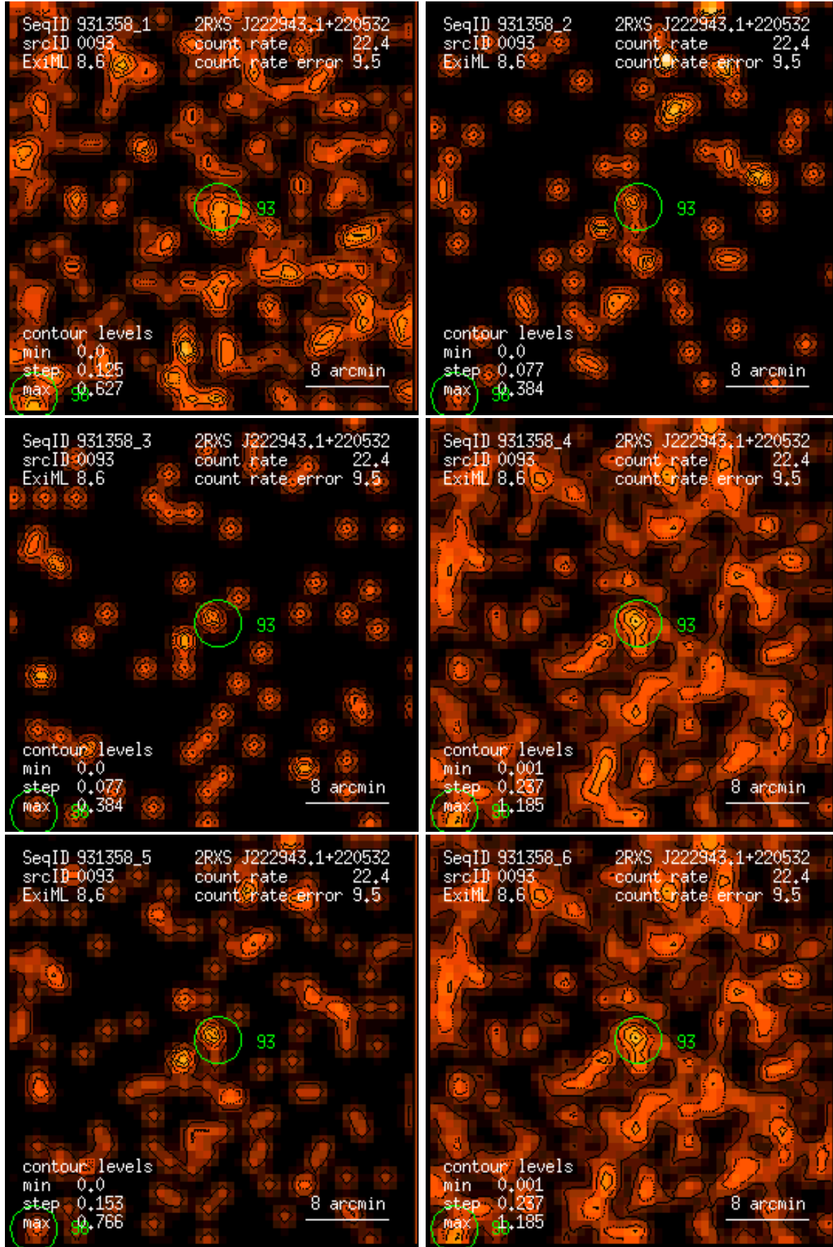
Figure 93: RASS 931358: detection 0093: band rate images, Gaussian filter: (1) PSPC channels 11 – 41, (2) 52 – 90, (3) 91 – 201, (4) 11 – 235, (5) 52 – 201, (6) 11 – 201. Broad band rates in counts/ks. Band rate contour levels in counts/ks/arcmin 2 .
