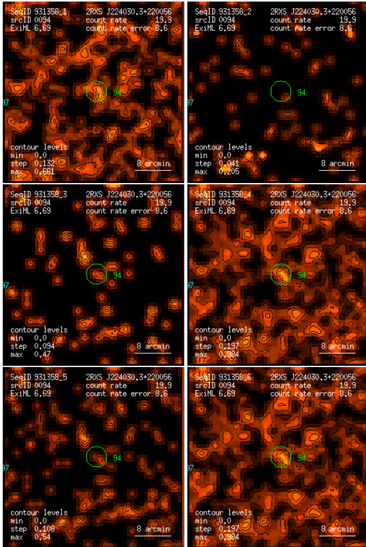
Figure 94: RASS 931358: detection 0094: band rate images, Gaussian filter: (1) PSPC channels 11 – 41, (2) 52 – 90, (3) 91 – 201, (4) 11 – 235, (5) 52 – 201, (6) 11 – 201. Broad band rates in counts/ks. Band rate contour levels in counts/ks/arcmin 2 .
