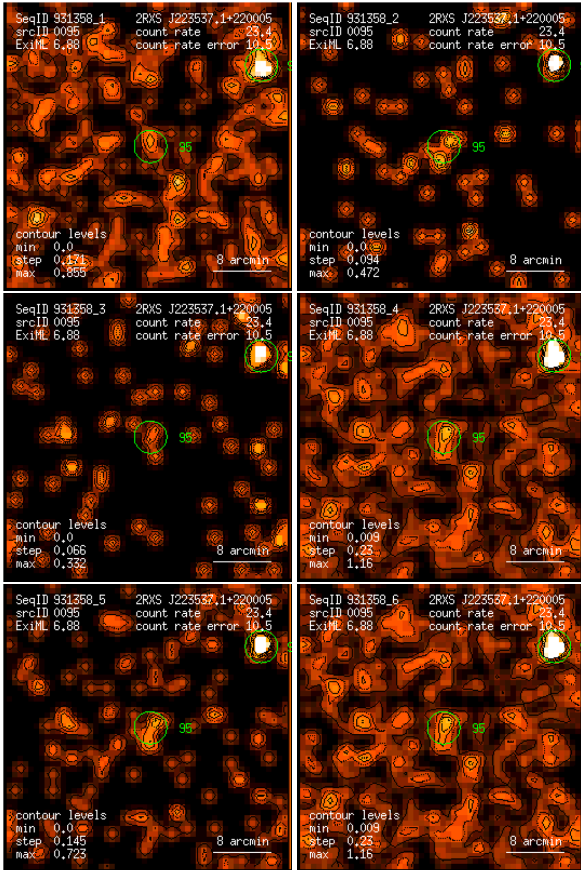
Figure 95: RASS 931358: detection 0095: band rate images, Gaussian filter: (1) PSPC channels 11 – 41, (2) 52 – 90, (3) 91 – 201, (4) 11 – 235, (5) 52 – 201, (6) 11 – 201. Broad band rates in counts/ks. Band rate contour levels in counts/ks/arcmin 2 .
