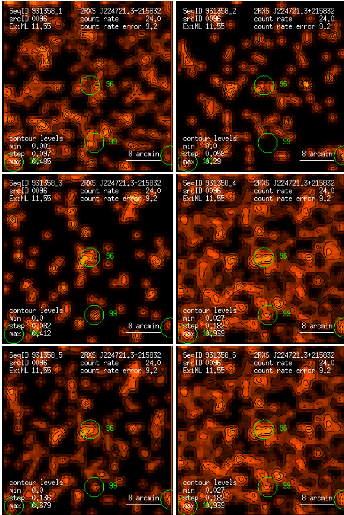
Figure 96: RASS 931358: detection 0096: band rate images, Gaussian filter: (1) PSPC channels 11 – 41, (2) 52 – 90, (3) 91 – 201, (4) 11 – 235, (5) 52 – 201, (6) 11 – 201. Broad band rates in counts/ks. Band rate contour levels in counts/ks/arcmin 2 .
