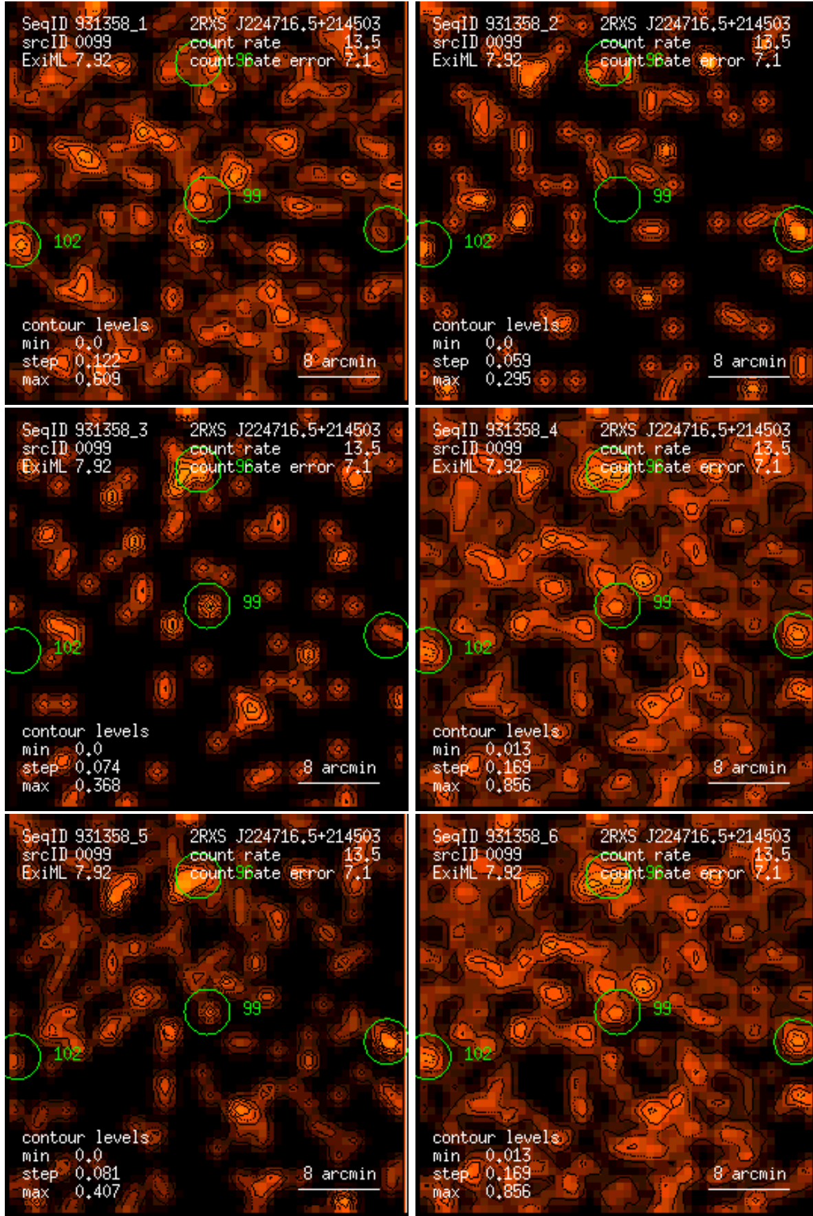
Figure 99: RASS 931358: detection 0099: band rate images, Gaussian filter: (1) PSPC channels 11 – 41, (2) 52 – 90, (3) 91 – 201, (4) 11 – 235, (5) 52 – 201, (6) 11 – 201. Broad band rates in counts/ks. Band rate contour levels in counts/ks/arcmin 2 .
