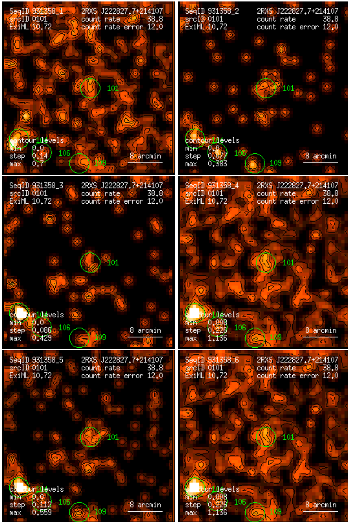
Figure 101: RASS 931358: detection 0101: band rate images, Gaussian filter: (1) PSPC channels 11 – 41, (2) 52 – 90, (3) 91 – 201, (4) 11 – 235, (5) 52 – 201, (6) 11 – 201. Broad band rates in counts/ks. Band rate contour levels in counts/ks/arcmin 2 .
