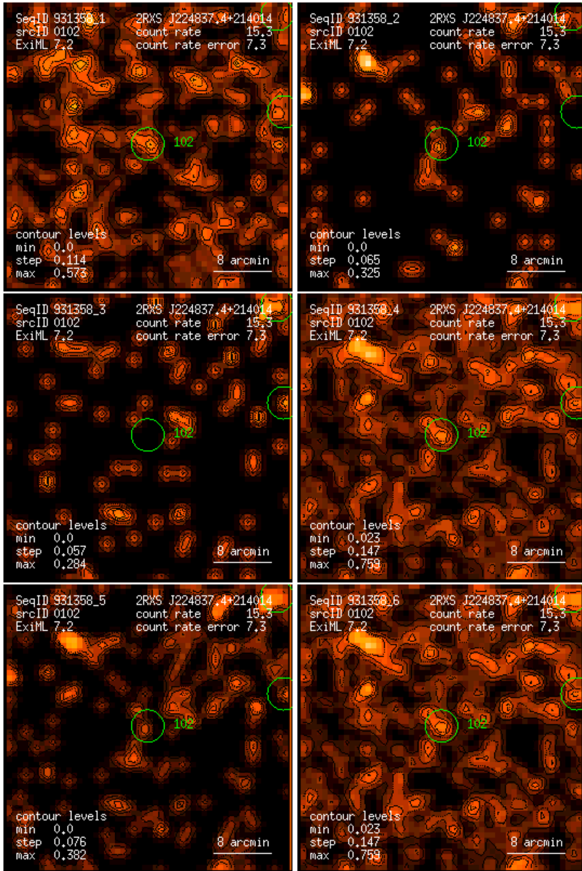
Figure 102: RASS 931358: detection 0102: band rate images, Gaussian filter: (1) PSPC channels 11 – 41, (2) 52 – 90, (3) 91 – 201, (4) 11 – 235, (5) 52 – 201, (6) 11 – 201. Broad band rates in counts/ks. Band rate contour levels in counts/ks/arcmin 2 .
