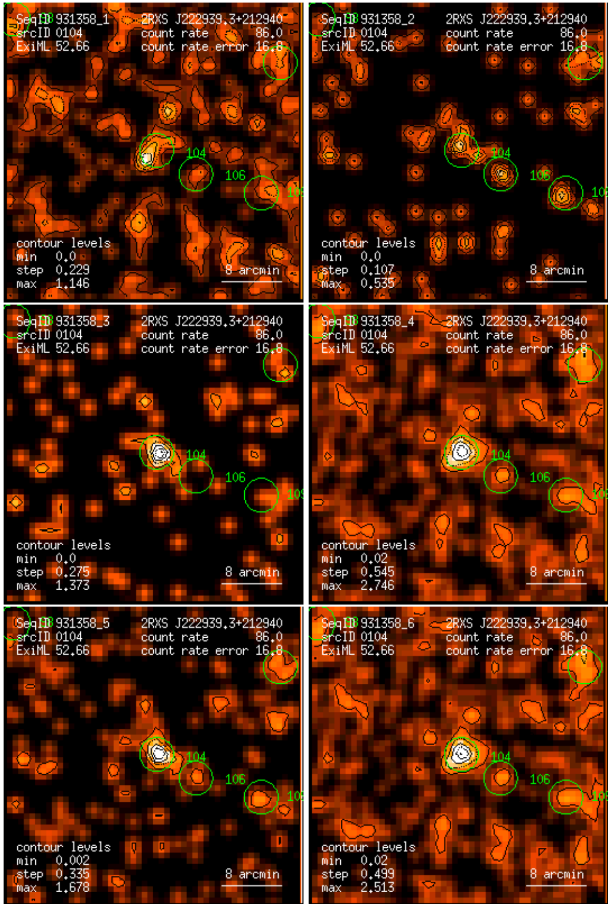
Figure 104: RASS 931358: detection 0104: band rate images, Gaussian filter: (1) PSPC channels 11 – 41, (2) 52 – 90, (3) 91 – 201, (4) 11 – 235, (5) 52 – 201, (6) 11 – 201. Broad band rates in counts/ks. Band rate contour levels in counts/ks/arcmin 2 .
