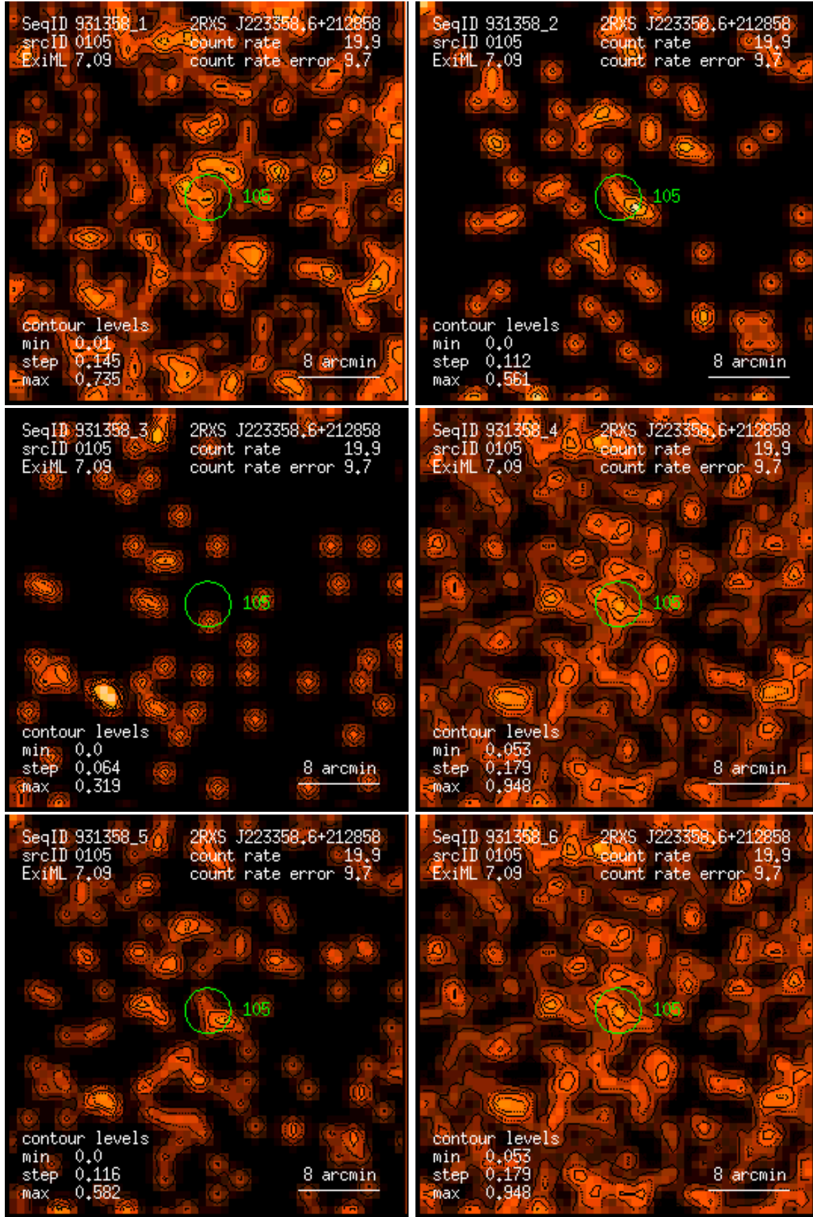
Figure 105: RASS 931358: detection 0105: band rate images, Gaussian filter: (1) PSPC channels 11 – 41, (2) 52 – 90, (3) 91 – 201, (4) 11 – 235, (5) 52 – 201, (6) 11 – 201. Broad band rates in counts/ks. Band rate contour levels in counts/ks/arcmin 2 .
