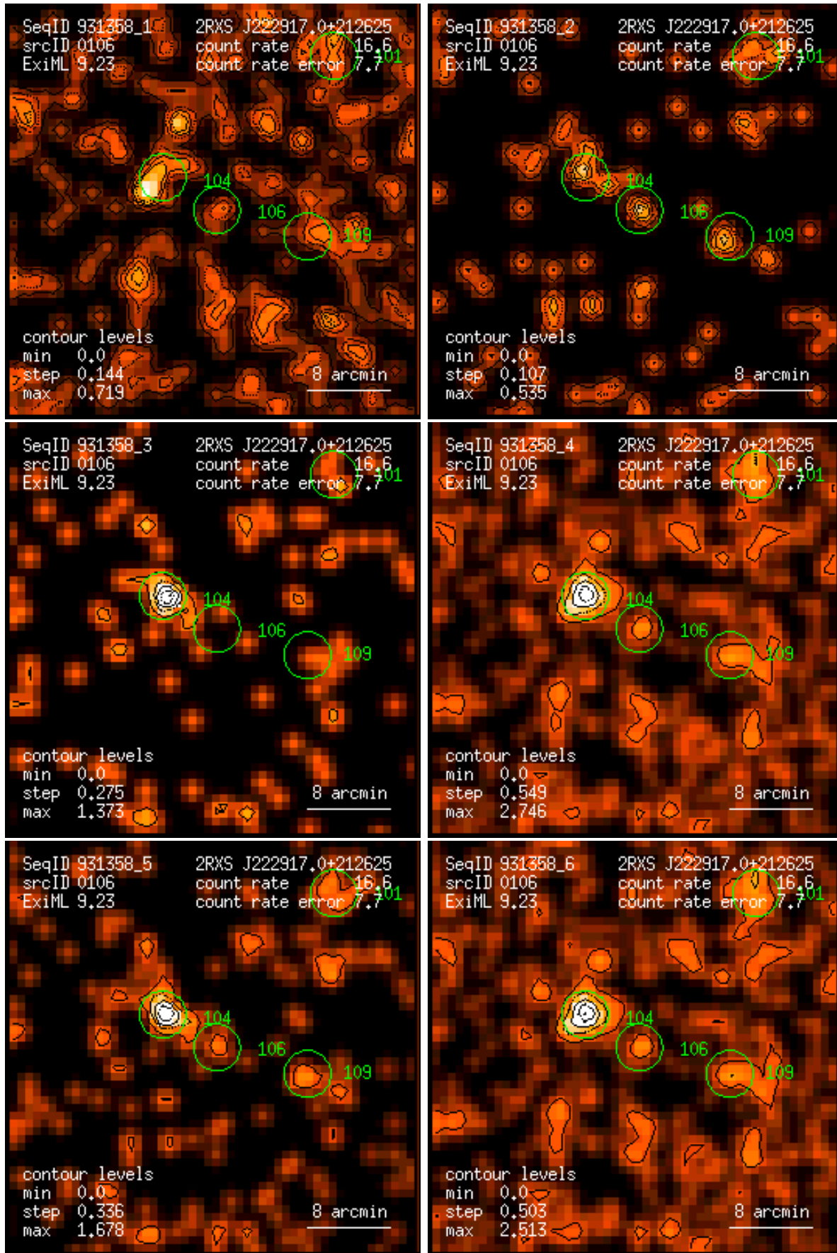
Figure 106: RASS 931358: detection 0106: band rate images, Gaussian filter: (1) PSPC channels 11 – 41, (2) 52 – 90, (3) 91 – 201, (4) 11 – 235, (5) 52 – 201, (6) 11 – 201. Broad band rates in counts/ks. Band rate contour levels in counts/ks/arcmin 2 .
